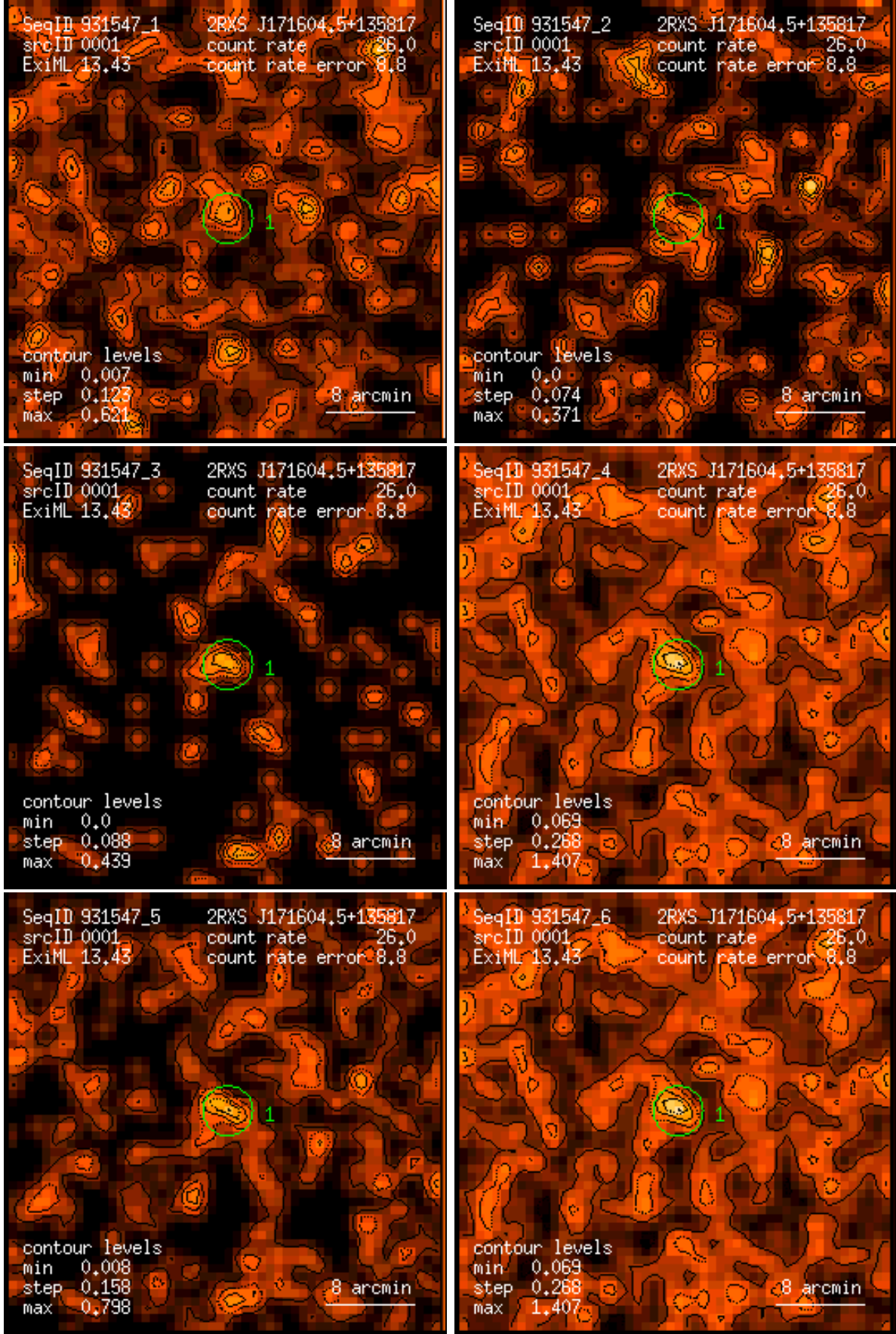
Figure 1: RASS 931547: detection 0001: band rate images, Gaussian filter: (1) PSPC channels 11 – 41, (2) 52 – 90, (3) 91 – 201, (4) 11 – 235, (5) 52 – 201, (6) 11 – 201. Broad band rates in counts/ks. Band rate contour levels in counts/ks/arcmin 2 .
