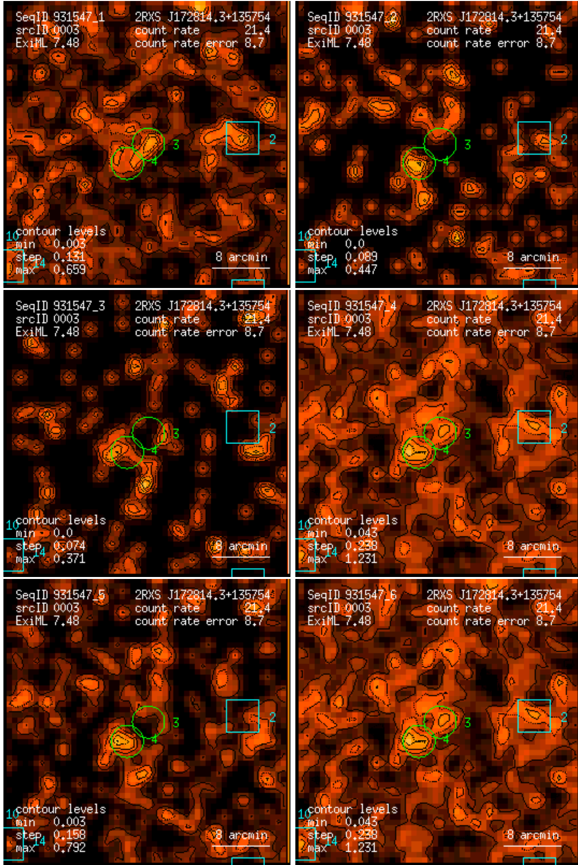
Figure 3: RASS 931547: detection 0003: band rate images, Gaussian filter: (1) PSPC channels 11 – 41, (2) 52 – 90, (3) 91 – 201, (4) 11 – 235, (5) 52 – 201, (6) 11 – 201. Broad band rates in counts/ks. Band rate contour levels in counts/ks/arcmin 2 .
