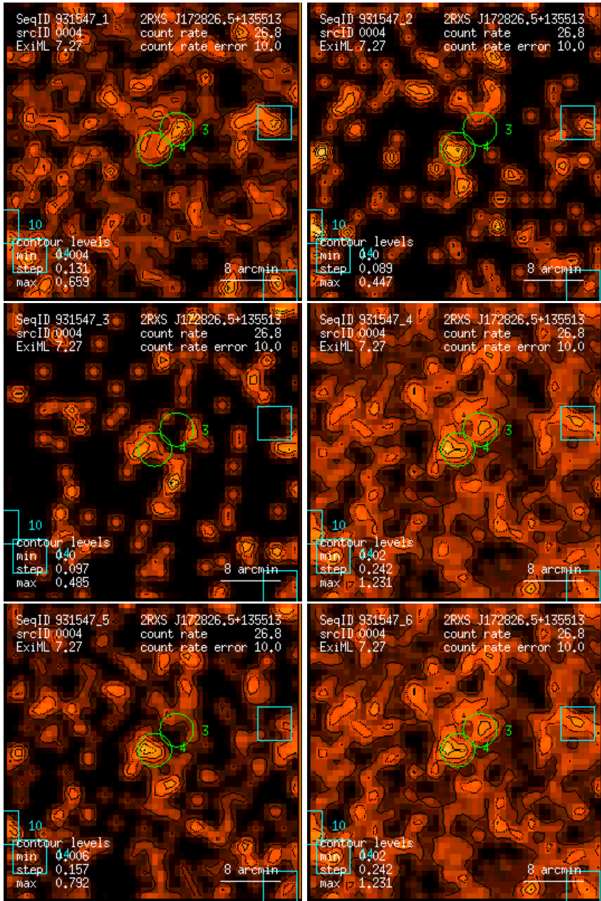
Figure 4: RASS 931547: detection 0004: band rate images, Gaussian filter: (1) PSPC channels 11 – 41, (2) 52 – 90, (3) 91 – 201, (4) 11 – 235, (5) 52 – 201, (6) 11 – 201. Broad band rates in counts/ks. Band rate contour levels in counts/ks/arcmin 2 .
