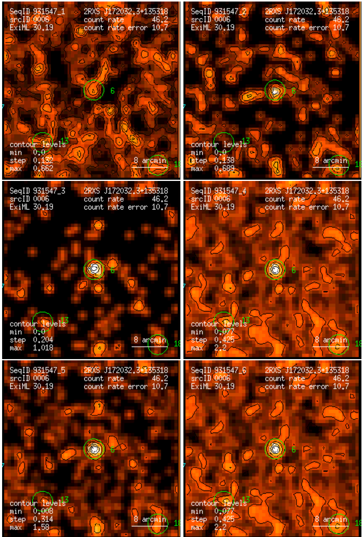
Figure 6: RASS 931547: detection 0006: band rate images, Gaussian filter: (1) PSPC channels 11 – 41, (2) 52 – 90, (3) 91 – 201, (4) 11 – 235, (5) 52 – 201, (6) 11 – 201. Broad band rates in counts/ks. Band rate contour levels in counts/ks/arcmin 2 .
