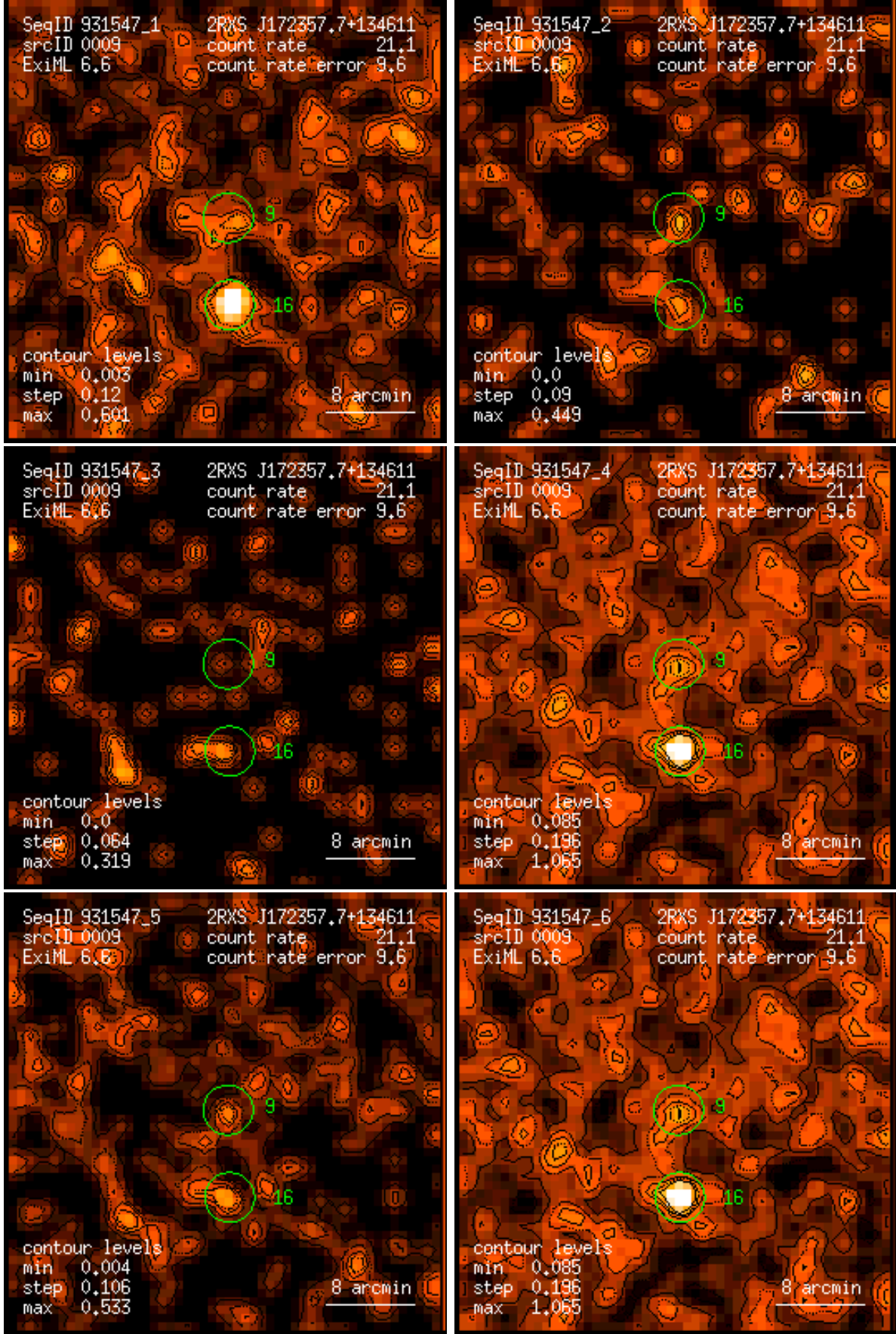
Figure 9: RASS 931547: detection 0009: band rate images, Gaussian filter: (1) PSPC channels 11 – 41, (2) 52 – 90, (3) 91 – 201, (4) 11 – 235, (5) 52 – 201, (6) 11 – 201. Broad band rates in counts/ks. Band rate contour levels in counts/ks/arcmin 2 .
