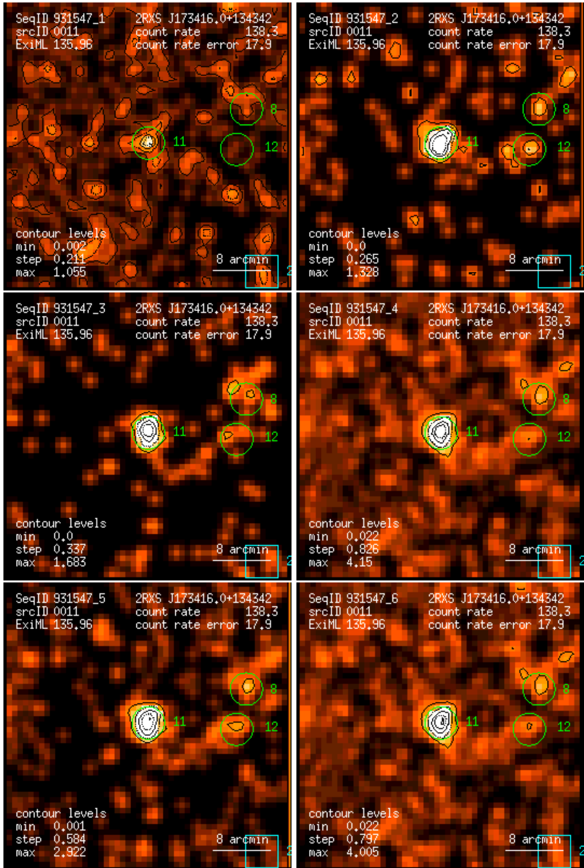
Figure 11: RASS 931547: detection 0011: band rate images, Gaussian filter: (1) PSPC channels 11 – 41, (2) 52 – 90, (3) 91 – 201, (4) 11 – 235, (5) 52 – 201, (6) 11 – 201. Broad band rates in counts/ks. Band rate contour levels in counts/ks/arcmin 2 .
