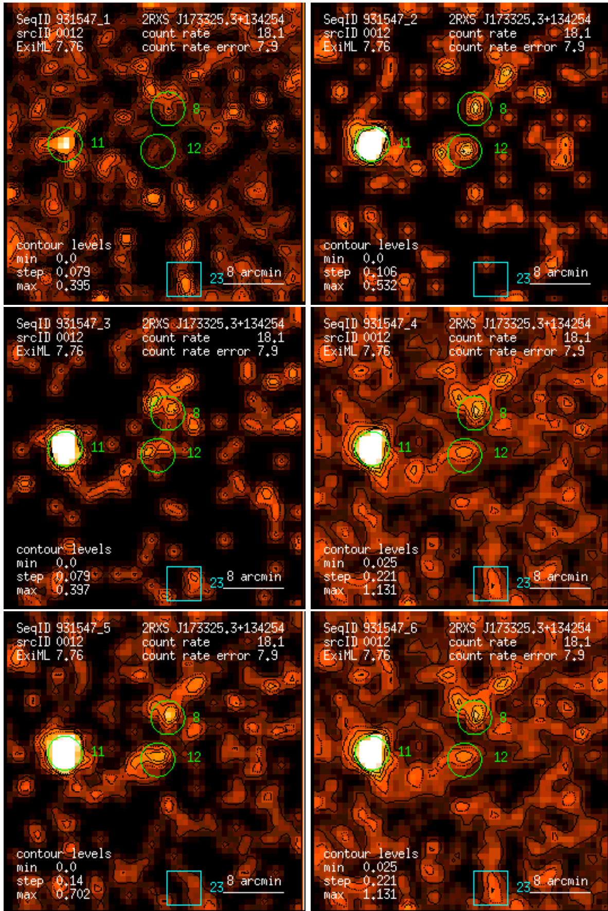
Figure 12: RASS 931547: detection 0012: band rate images, Gaussian filter: (1) PSPC channels 11 – 41, (2) 52 – 90, (3) 91 – 201, (4) 11 – 235, (5) 52 – 201, (6) 11 – 201. Broad band rates in counts/ks. Band rate contour levels in counts/ks/arcmin 2 .
