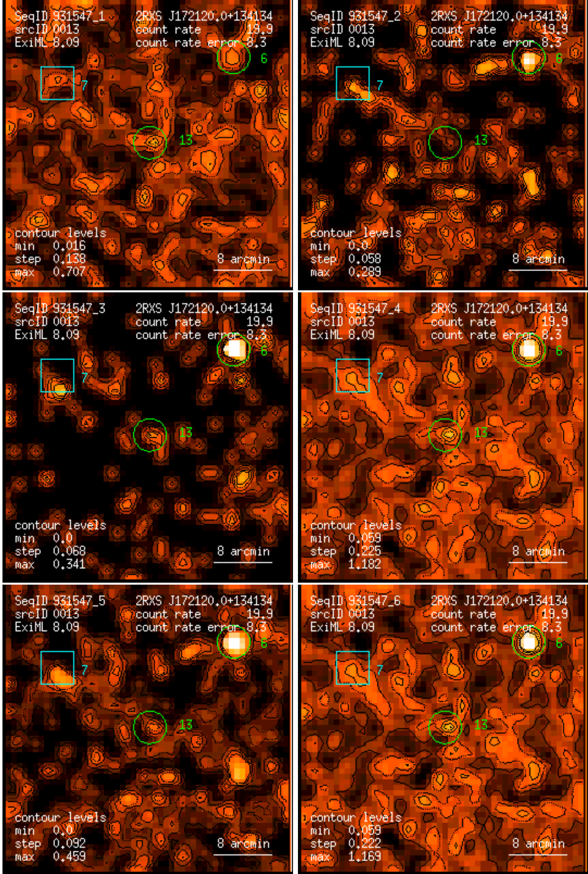
Figure 13: RASS 931547: detection 0013: band rate images, Gaussian filter: (1) PSPC channels 11 – 41, (2) 52 – 90, (3) 91 – 201, (4) 11 – 235, (5) 52 – 201, (6) 11 – 201. Broad band rates in counts/ks. Band rate contour levels in counts/ks/arcmin 2 .
