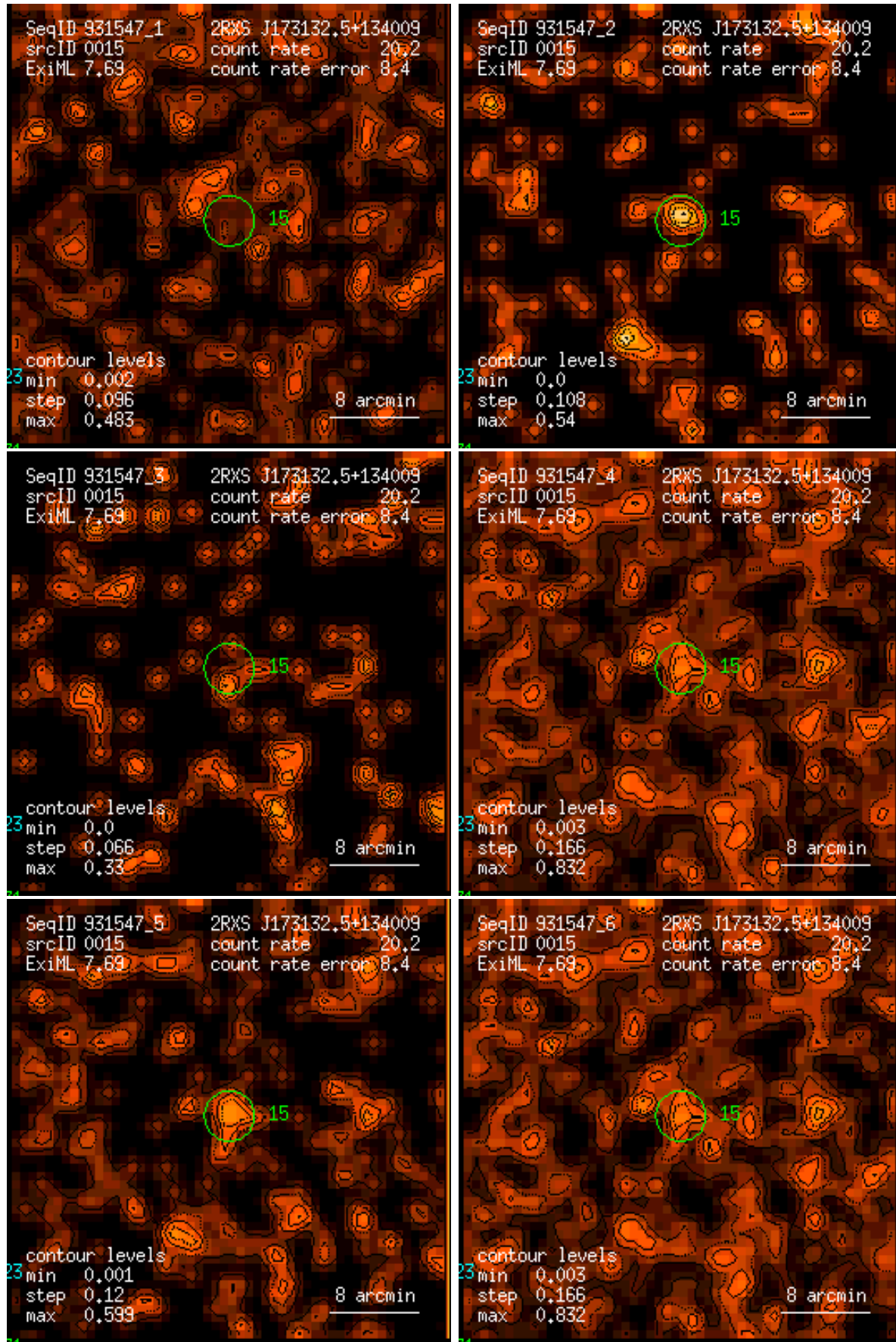
Figure 15: RASS 931547: detection 0015: band rate images, Gaussian filter: (1) PSPC channels 11 – 41, (2) 52 – 90, (3) 91 – 201, (4) 11 – 235, (5) 52 – 201, (6) 11 – 201. Broad band rates in counts/ks. Band rate contour levels in counts/ks/arcmin 2 .
