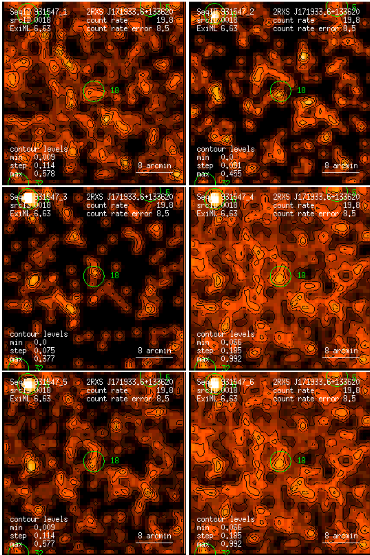
Figure 18: RASS 931547: detection 0018: band rate images, Gaussian filter: (1) PSPC channels 11 – 41, (2) 52 – 90, (3) 91 – 201, (4) 11 – 235, (5) 52 – 201, (6) 11 – 201. Broad band rates in counts/ks. Band rate contour levels in counts/ks/arcmin 2 .
