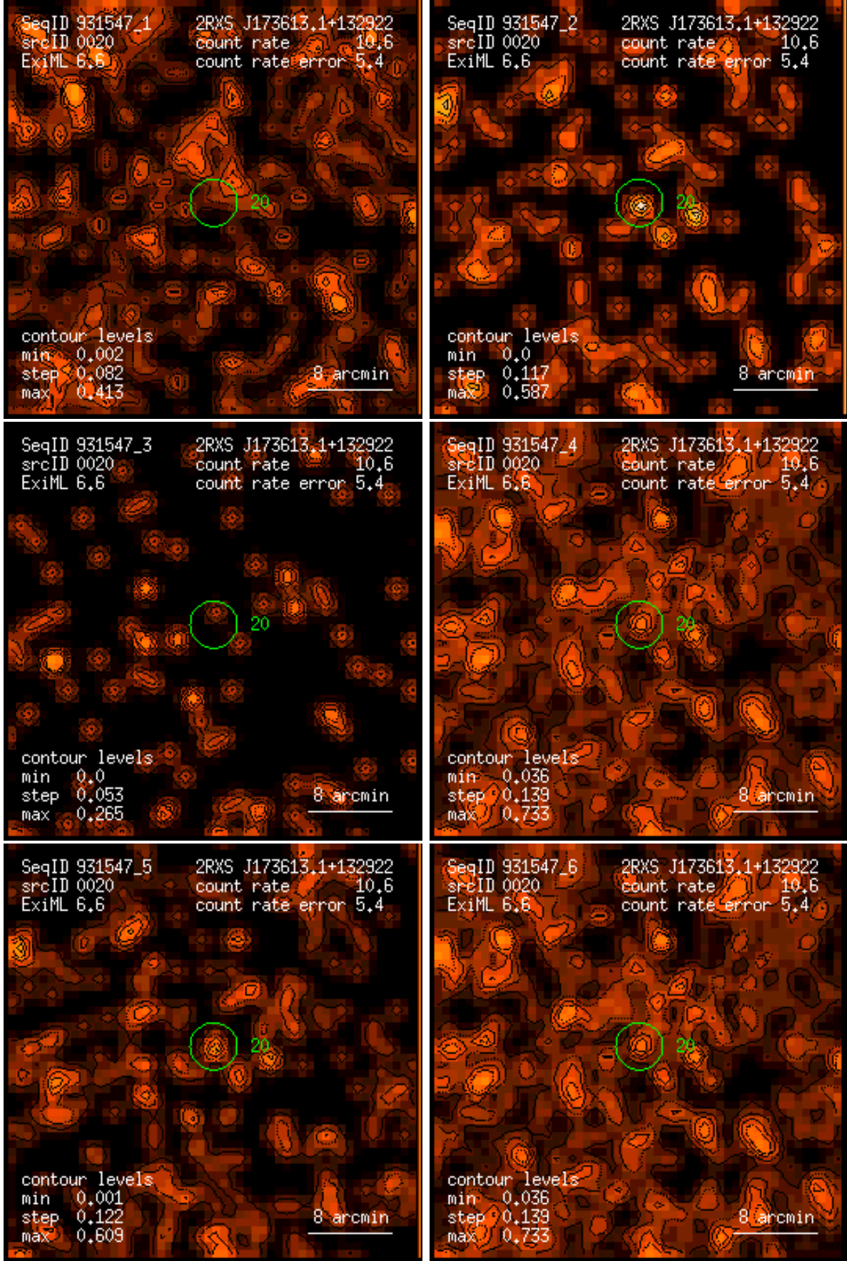
Figure 20: RASS 931547: detection 0020: band rate images, Gaussian filter: (1) PSPC channels 11 – 41, (2) 52 – 90, (3) 91 – 201, (4) 11 – 235, (5) 52 – 201, (6) 11 – 201. Broad band rates in counts/ks. Band rate contour levels in counts/ks/arcmin 2 .
