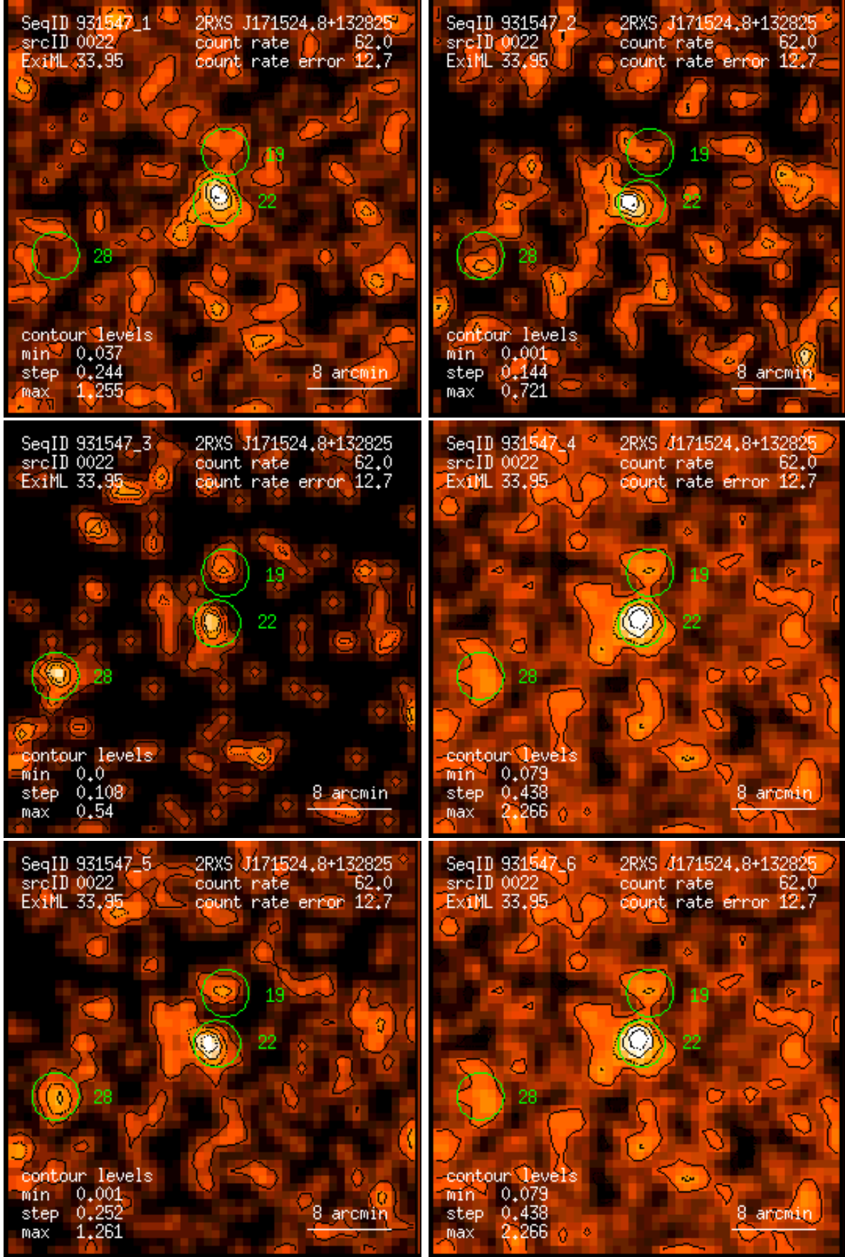
Figure 22: RASS 931547: detection 0022: band rate images, Gaussian filter: (1) PSPC channels 11 – 41, (2) 52 – 90, (3) 91 – 201, (4) 11 – 235, (5) 52 – 201, (6) 11 – 201. Broad band rates in counts/ks. Band rate contour levels in counts/ks/arcmin 2 .
