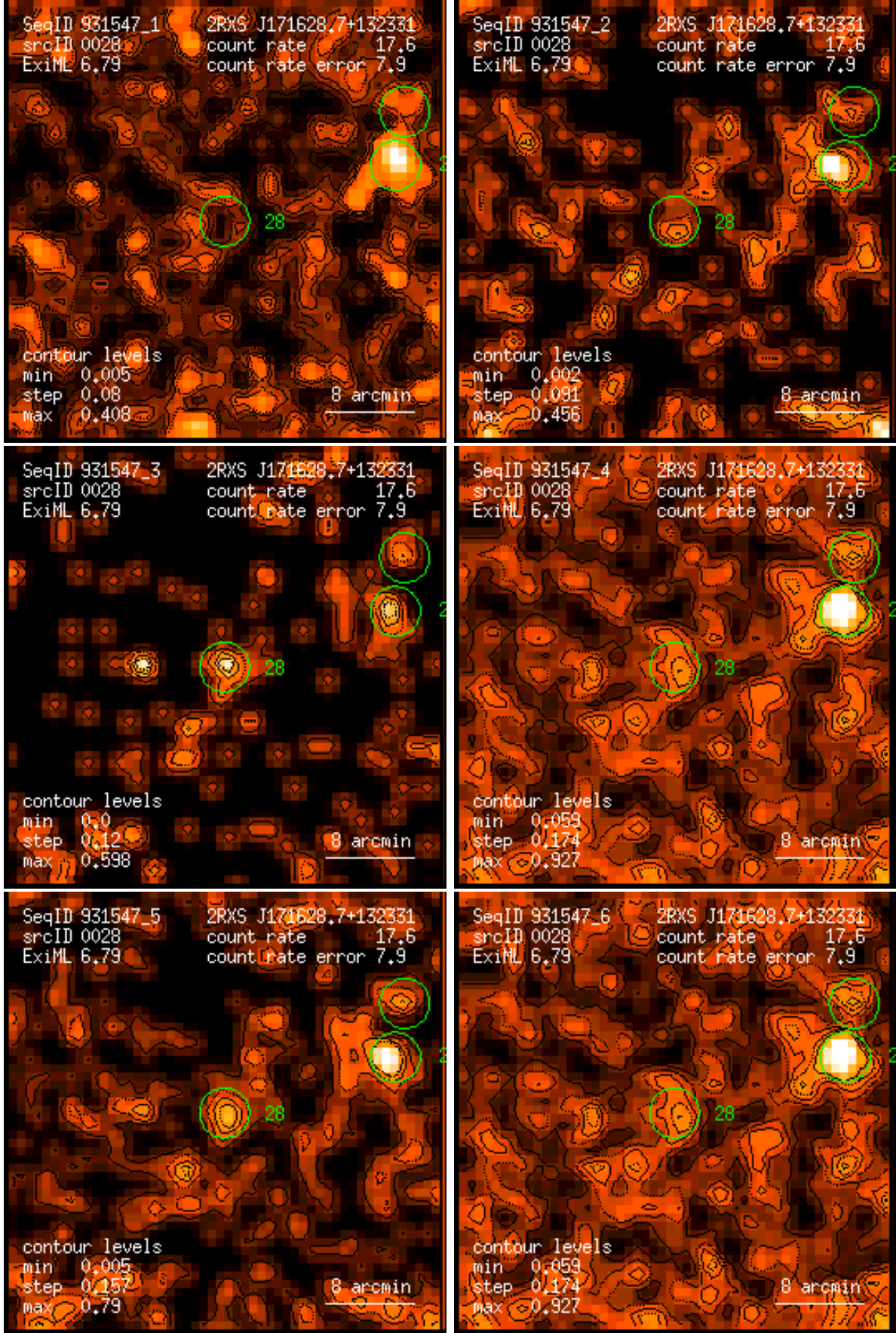
Figure 28: RASS 931547: detection 0028: band rate images, Gaussian filter: (1) PSPC channels 11 – 41, (2) 52 – 90, (3) 91 – 201, (4) 11 – 235, (5) 52 – 201, (6) 11 – 201. Broad band rates in counts/ks. Band rate contour levels in counts/ks/arcmin 2 .
