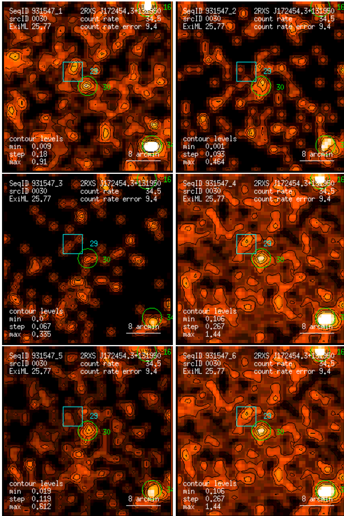
Figure 30: RASS 931547: detection 0030: band rate images, Gaussian filter: (1) PSPC channels 11 – 41, (2) 52 – 90, (3) 91 – 201, (4) 11 – 235, (5) 52 – 201, (6) 11 – 201. Broad band rates in counts/ks. Band rate contour levels in counts/ks/arcmin 2 .
