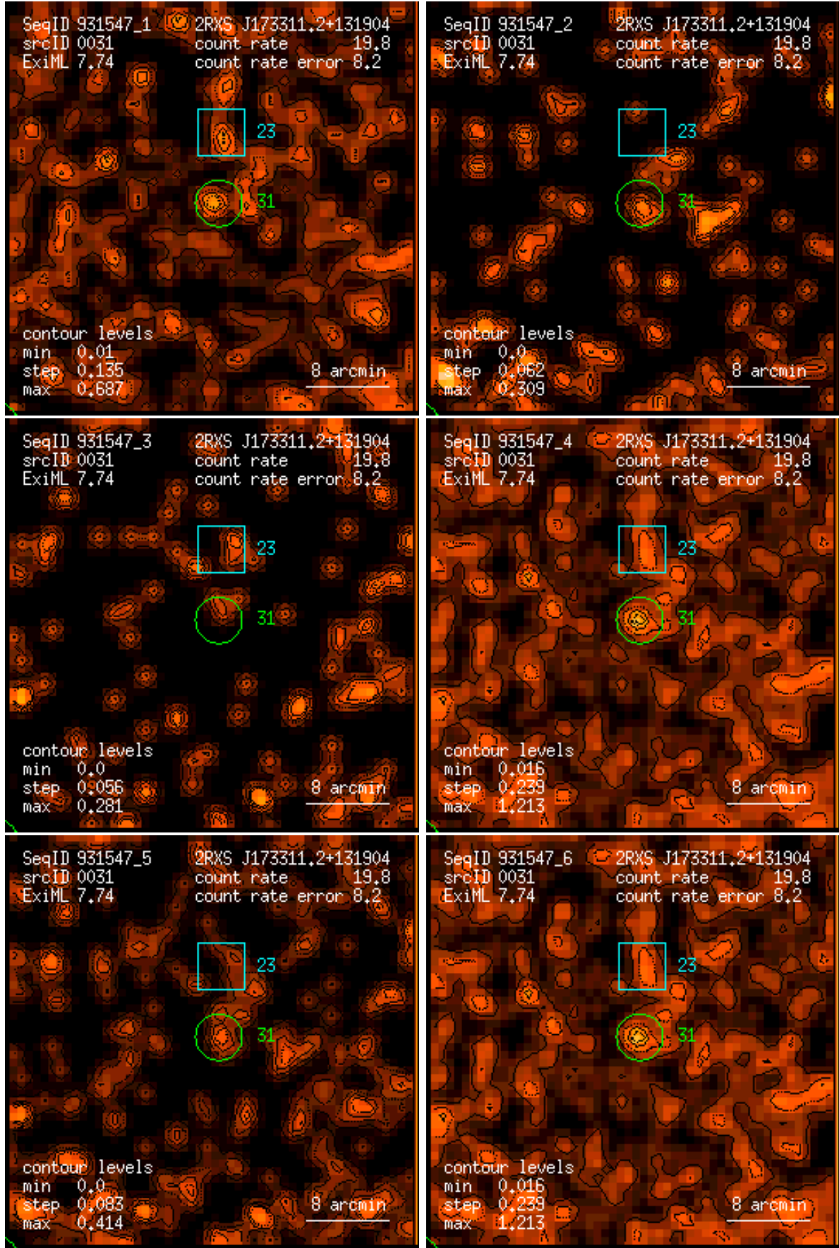
Figure 31: RASS 931547: detection 0031: band rate images, Gaussian filter: (1) PSPC channels 11 – 41, (2) 52 – 90, (3) 91 – 201, (4) 11 – 235, (5) 52 – 201, (6) 11 – 201. Broad band rates in counts/ks. Band rate contour levels in counts/ks/arcmin 2 .
