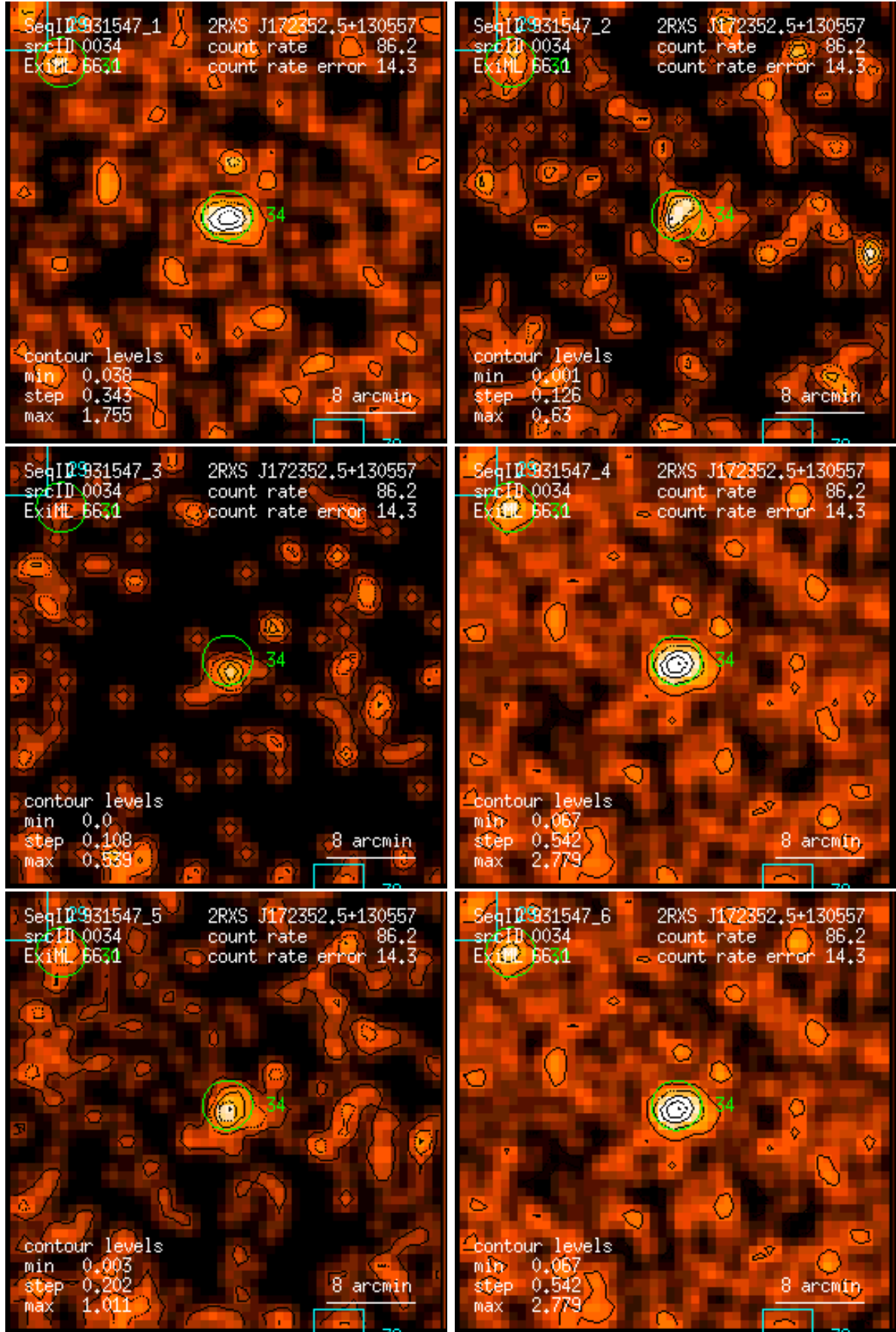
Figure 34: RASS 931547: detection 0034: band rate images, Gaussian filter: (1) PSPC channels 11 – 41, (2) 52 – 90, (3) 91 – 201, (4) 11 – 235, (5) 52 – 201, (6) 11 – 201. Broad band rates in counts/ks. Band rate contour levels in counts/ks/arcmin 2 .
