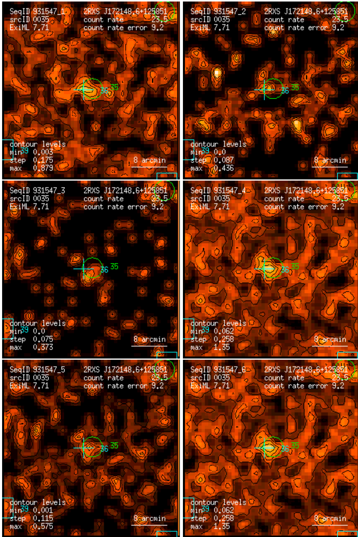
Figure 35: RASS 931547: detection 0035: band rate images, Gaussian filter: (1) PSPC channels 11 – 41, (2) 52 – 90, (3) 91 – 201, (4) 11 – 235, (5) 52 – 201, (6) 11 – 201. Broad band rates in counts/ks. Band rate contour levels in counts/ks/arcmin 2 .
