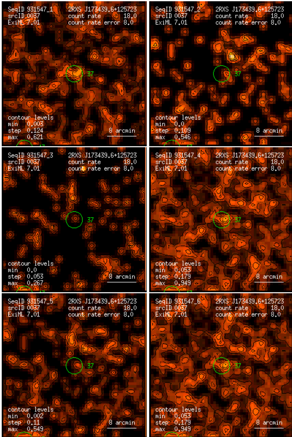
Figure 37: RASS 931547: detection 0037: band rate images, Gaussian filter: (1) PSPC channels 11 – 41, (2) 52 – 90, (3) 91 – 201, (4) 11 – 235, (5) 52 – 201, (6) 11 – 201. Broad band rates in counts/ks. Band rate contour levels in counts/ks/arcmin 2 .
