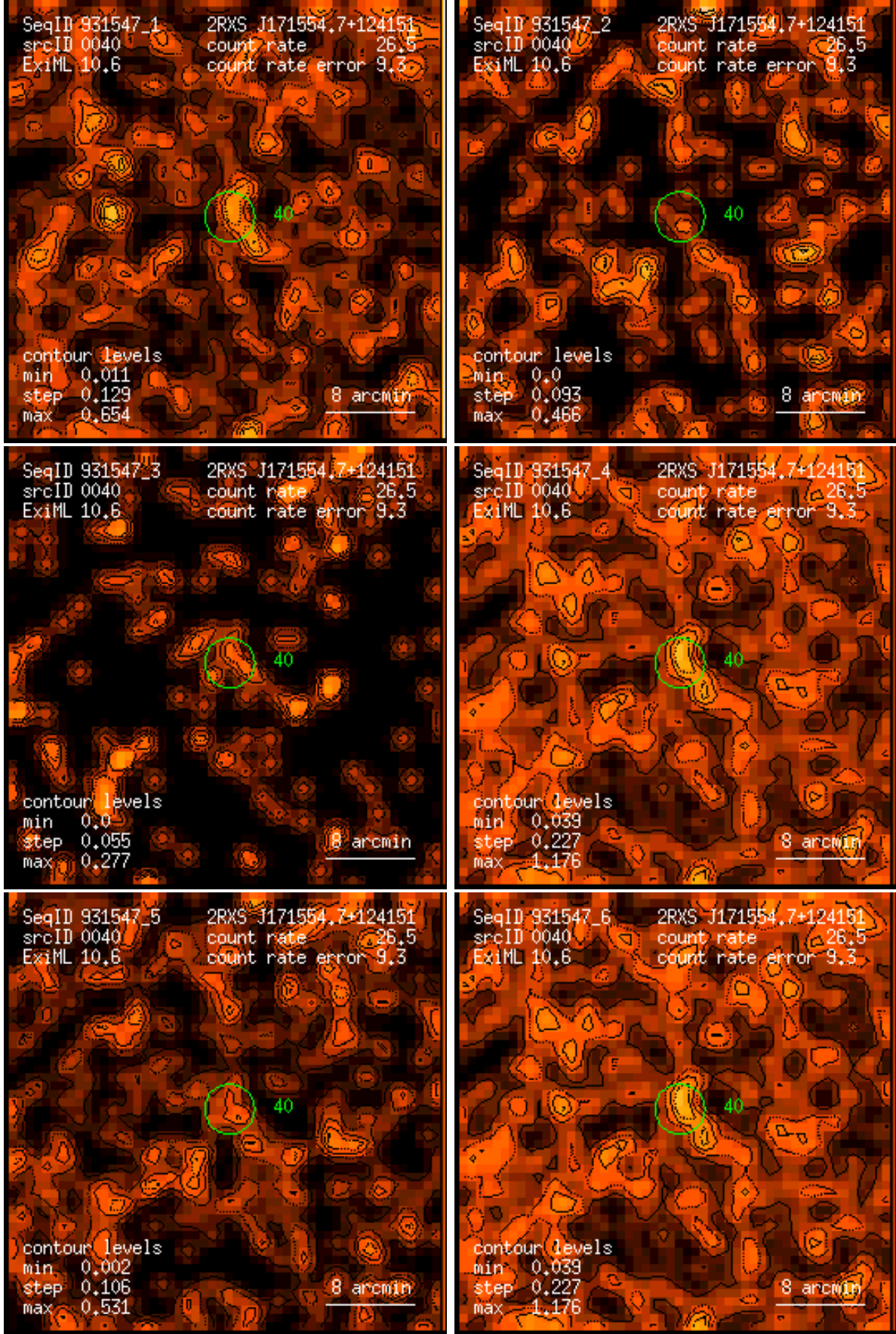
Figure 40: RASS 931547: detection 0040: band rate images, Gaussian filter: (1) PSPC channels 11 – 41, (2) 52 – 90, (3) 91 – 201, (4) 11 – 235, (5) 52 – 201, (6) 11 – 201. Broad band rates in counts/ks. Band rate contour levels in counts/ks/arcmin 2 .
