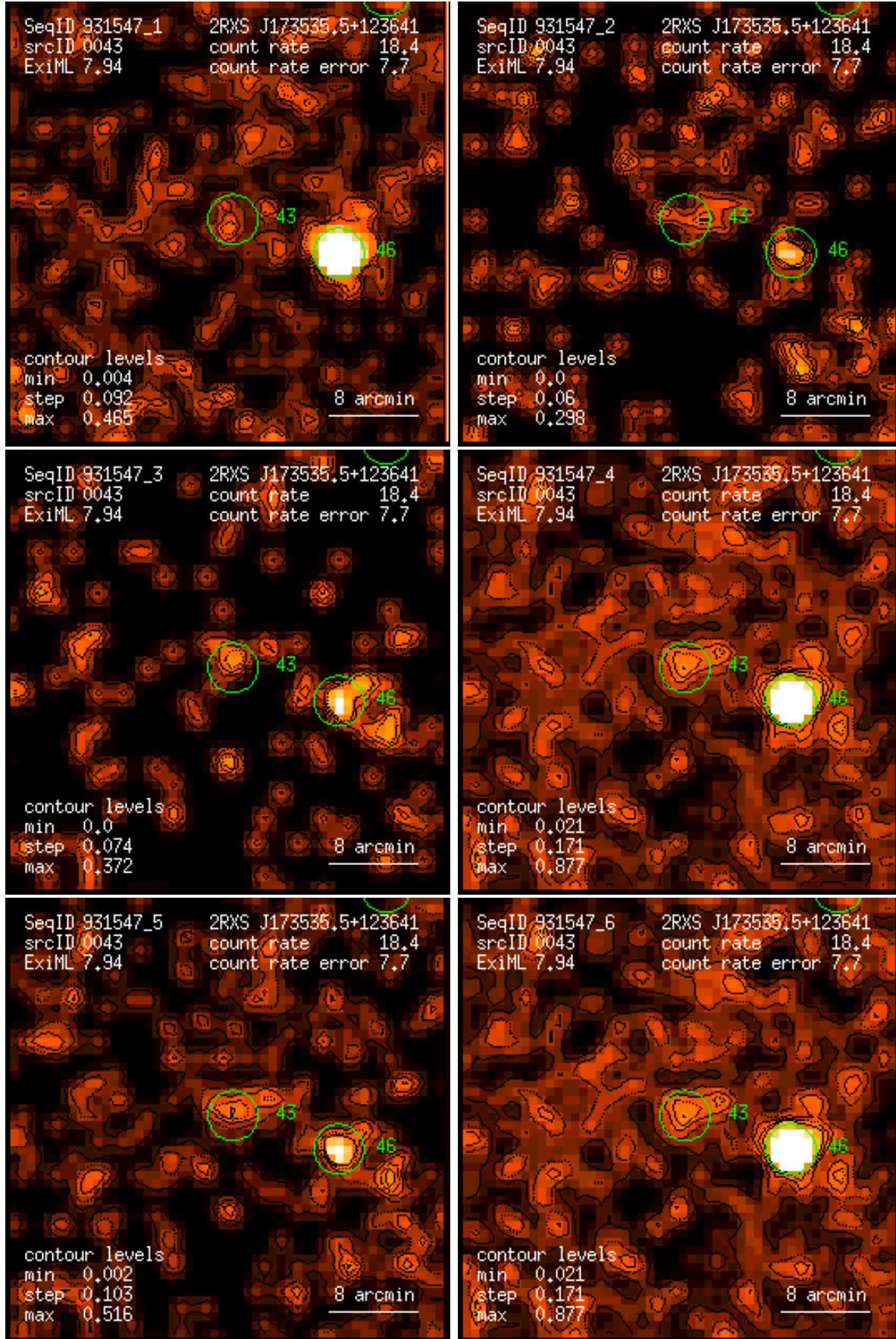
Figure 43: RASS 931547: detection 0043: band rate images, Gaussian filter: (1) PSPC channels 11 – 41, (2) 52 – 90, (3) 91 – 201, (4) 11 – 235, (5) 52 – 201, (6) 11 – 201. Broad band rates in counts/ks. Band rate contour levels in counts/ks/arcmin 2 .
