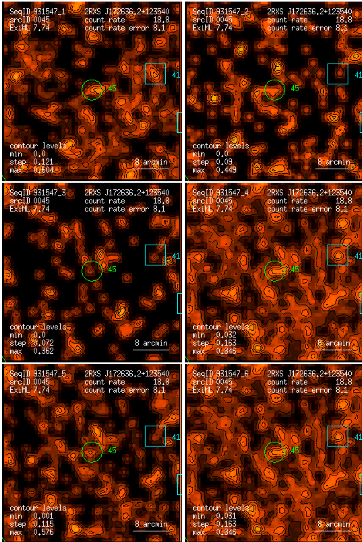
Figure 45: RASS 931547: detection 0045: band rate images, Gaussian filter: (1) PSPC channels 11 – 41, (2) 52 – 90, (3) 91 – 201, (4) 11 – 235, (5) 52 – 201, (6) 11 – 201. Broad band rates in counts/ks. Band rate contour levels in counts/ks/arcmin 2 .
