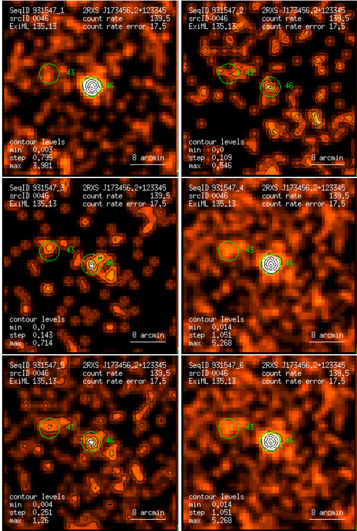
Figure 46: RASS 931547: detection 0046: band rate images, Gaussian filter: (1) PSPC channels 11 – 41, (2) 52 – 90, (3) 91 – 201, (4) 11 – 235, (5) 52 – 201, (6) 11 – 201. Broad band rates in counts/ks. Band rate contour levels in counts/ks/arcmin 2 .
