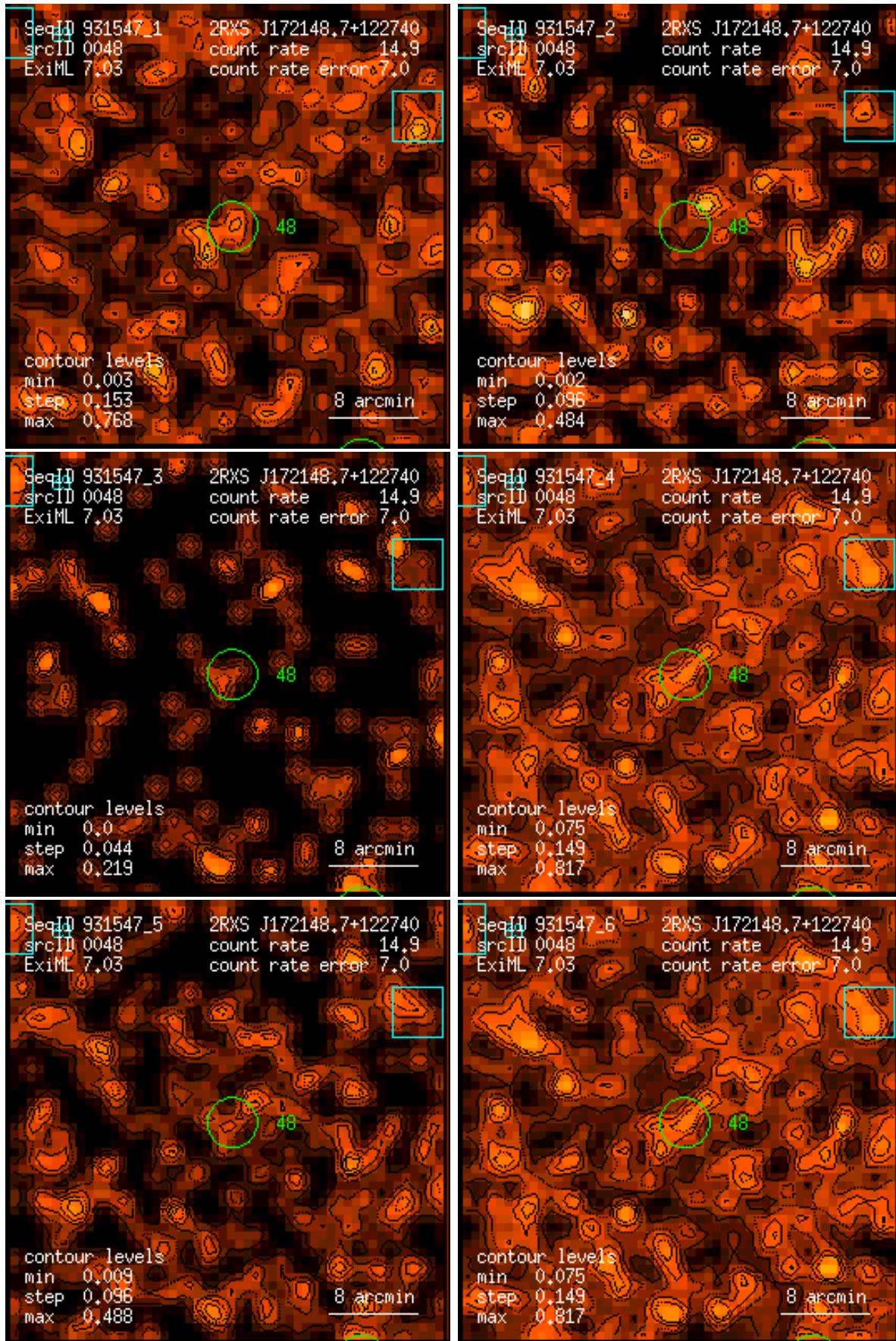
Figure 48: RASS 931547: detection 0048: band rate images, Gaussian filter: (1) PSPC channels 11 – 41, (2) 52 – 90, (3) 91 – 201, (4) 11 – 235, (5) 52 – 201, (6) 11 – 201. Broad band rates in counts/ks. Band rate contour levels in counts/ks/arcmin 2 .
