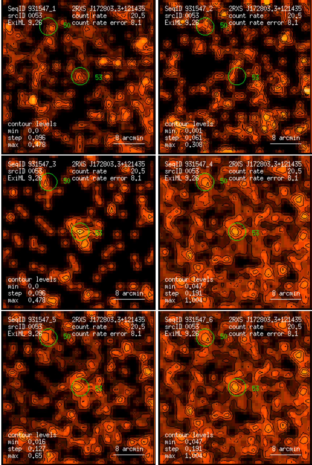
Figure 53: RASS 931547: detection 0053: band rate images, Gaussian filter: (1) PSPC channels 11 – 41, (2) 52 – 90, (3) 91 – 201, (4) 11 – 235, (5) 52 – 201, (6) 11 – 201. Broad band rates in counts/ks. Band rate contour levels in counts/ks/arcmin 2 .
