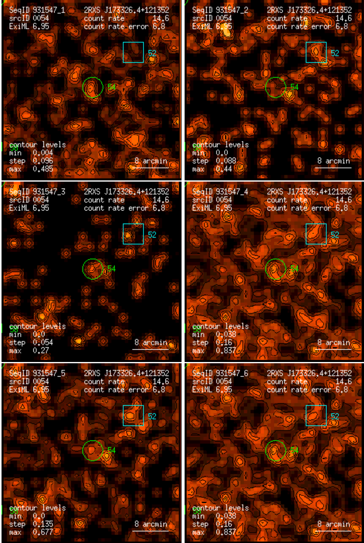
Figure 54: RASS 931547: detection 0054: band rate images, Gaussian filter: (1) PSPC channels 11 – 41, (2) 52 – 90, (3) 91 – 201, (4) 11 – 235, (5) 52 – 201, (6) 11 – 201. Broad band rates in counts/ks. Band rate contour levels in counts/ks/arcmin 2 .
