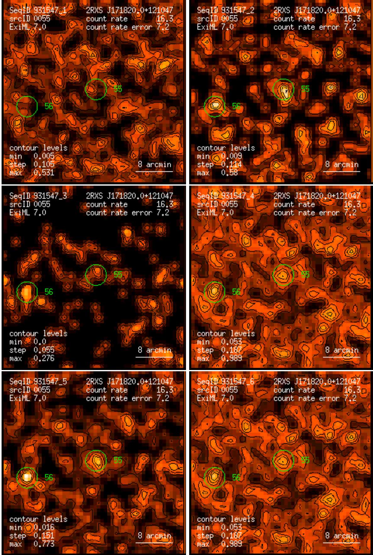
Figure 55: RASS 931547: detection 0055: band rate images, Gaussian filter: (1) PSPC channels 11 – 41, (2) 52 – 90, (3) 91 – 201, (4) 11 – 235, (5) 52 – 201, (6) 11 – 201. Broad band rates in counts/ks. Band rate contour levels in counts/ks/arcmin 2 .
