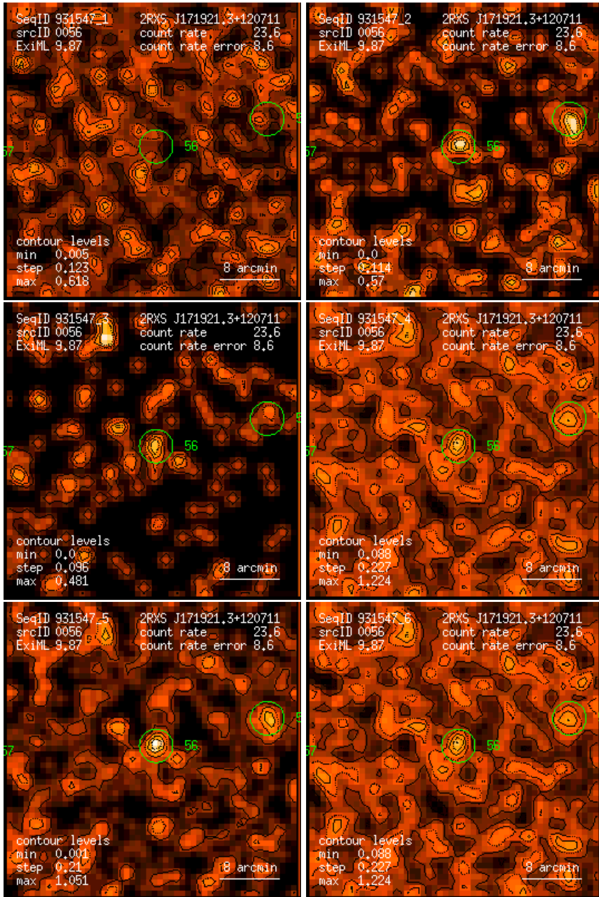
Figure 56: RASS 931547: detection 0056: band rate images, Gaussian filter: (1) PSPC channels 11 – 41, (2) 52 – 90, (3) 91 – 201, (4) 11 – 235, (5) 52 – 201, (6) 11 – 201. Broad band rates in counts/ks. Band rate contour levels in counts/ks/arcmin 2 .
