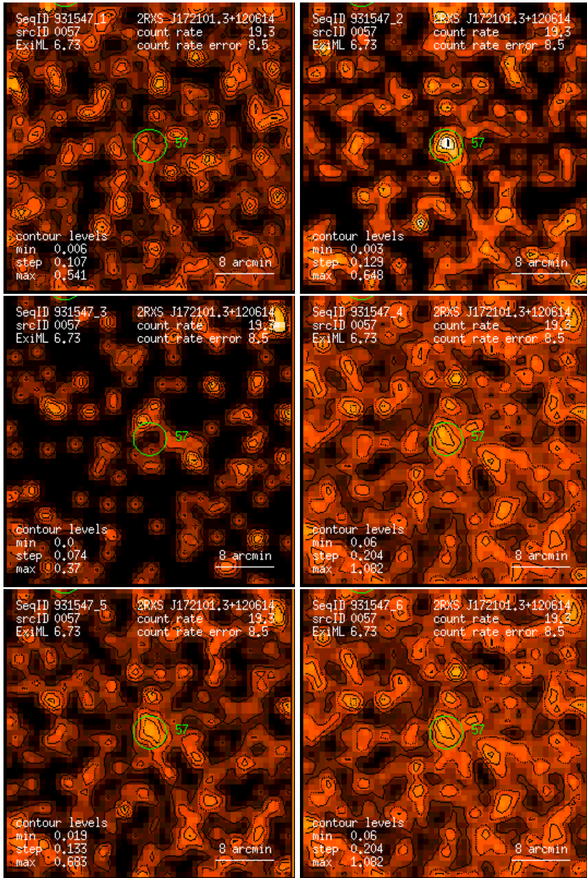
Figure 57: RASS 931547: detection 0057: band rate images, Gaussian filter: (1) PSPC channels 11 – 41, (2) 52 – 90, (3) 91 – 201, (4) 11 – 235, (5) 52 – 201, (6) 11 – 201. Broad band rates in counts/ks. Band rate contour levels in counts/ks/arcmin 2 .
