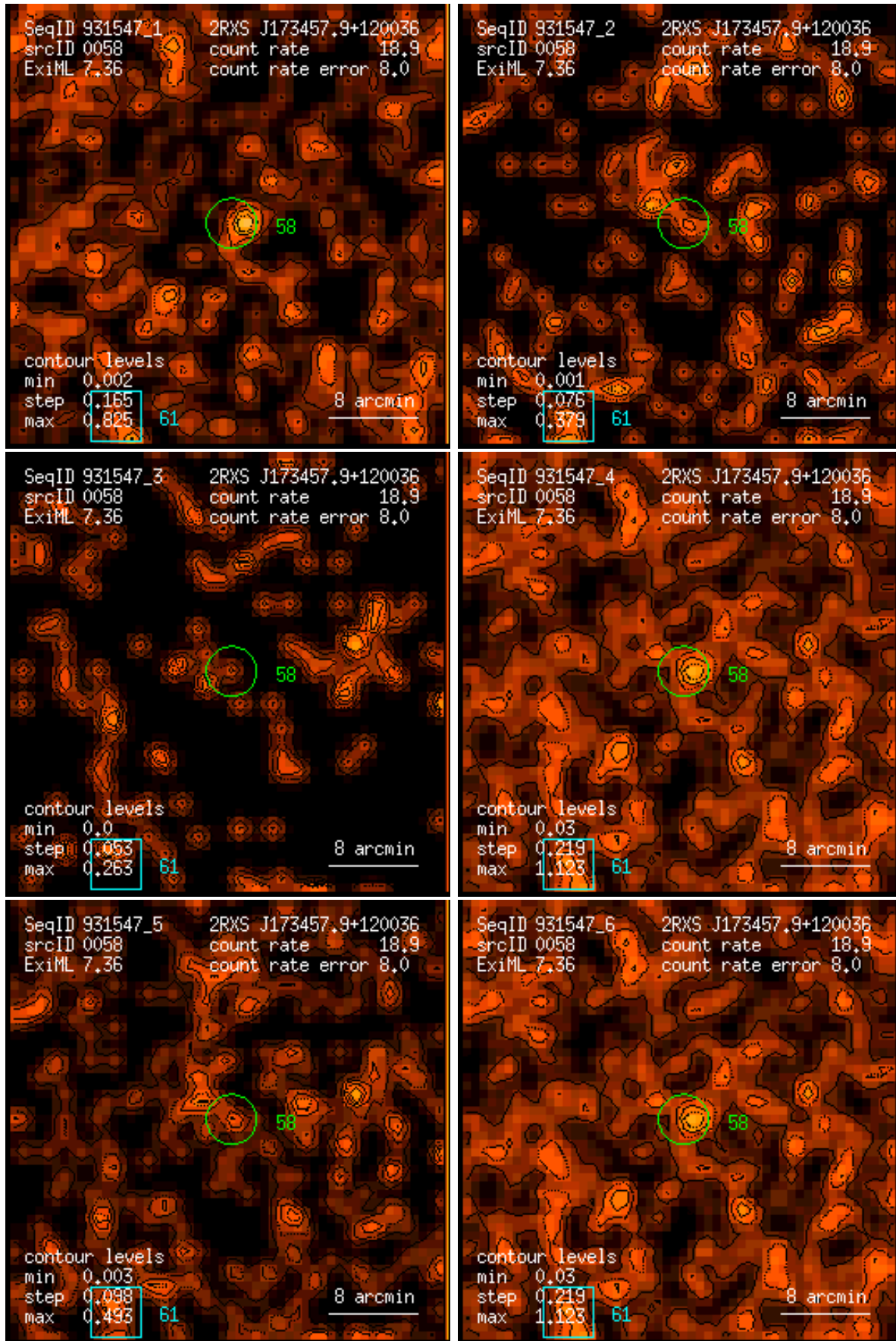
Figure 58: RASS 931547: detection 0058: band rate images, Gaussian filter: (1) PSPC channels 11 – 41, (2) 52 – 90, (3) 91 – 201, (4) 11 – 235, (5) 52 – 201, (6) 11 – 201. Broad band rates in counts/ks. Band rate contour levels in counts/ks/arcmin 2 .
