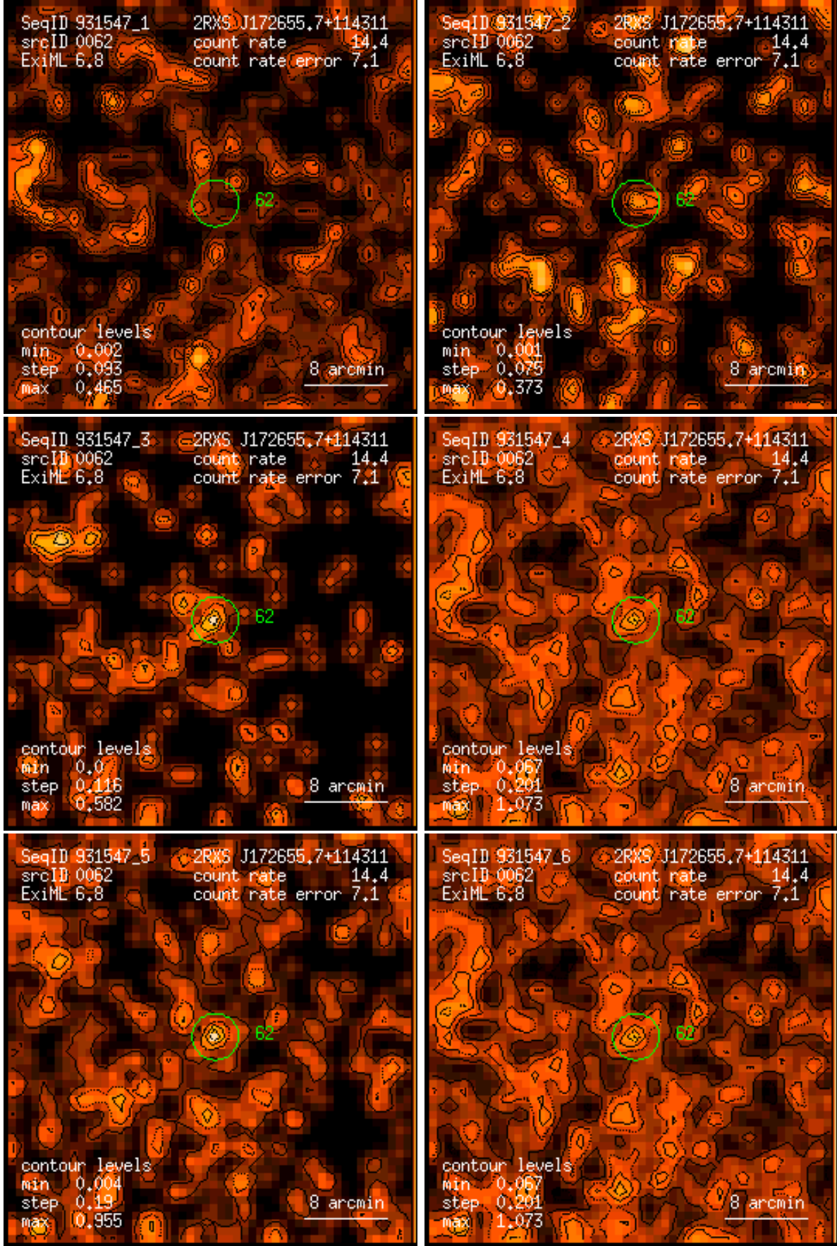
Figure 62: RASS 931547: detection 0062: band rate images, Gaussian filter: (1) PSPC channels 11 – 41, (2) 52 – 90, (3) 91 – 201, (4) 11 – 235, (5) 52 – 201, (6) 11 – 201. Broad band rates in counts/ks. Band rate contour levels in counts/ks/arcmin 2 .
