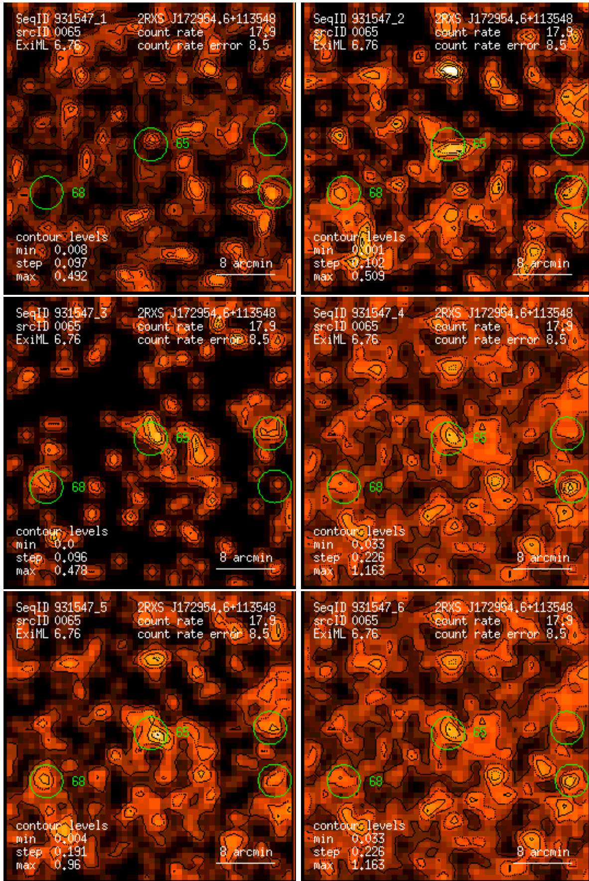
Figure 65: RASS 931547: detection 0065: band rate images, Gaussian filter: (1) PSPC channels 11 – 41, (2) 52 – 90, (3) 91 – 201, (4) 11 – 235, (5) 52 – 201, (6) 11 – 201. Broad band rates in counts/ks. Band rate contour levels in counts/ks/arcmin 2 .
