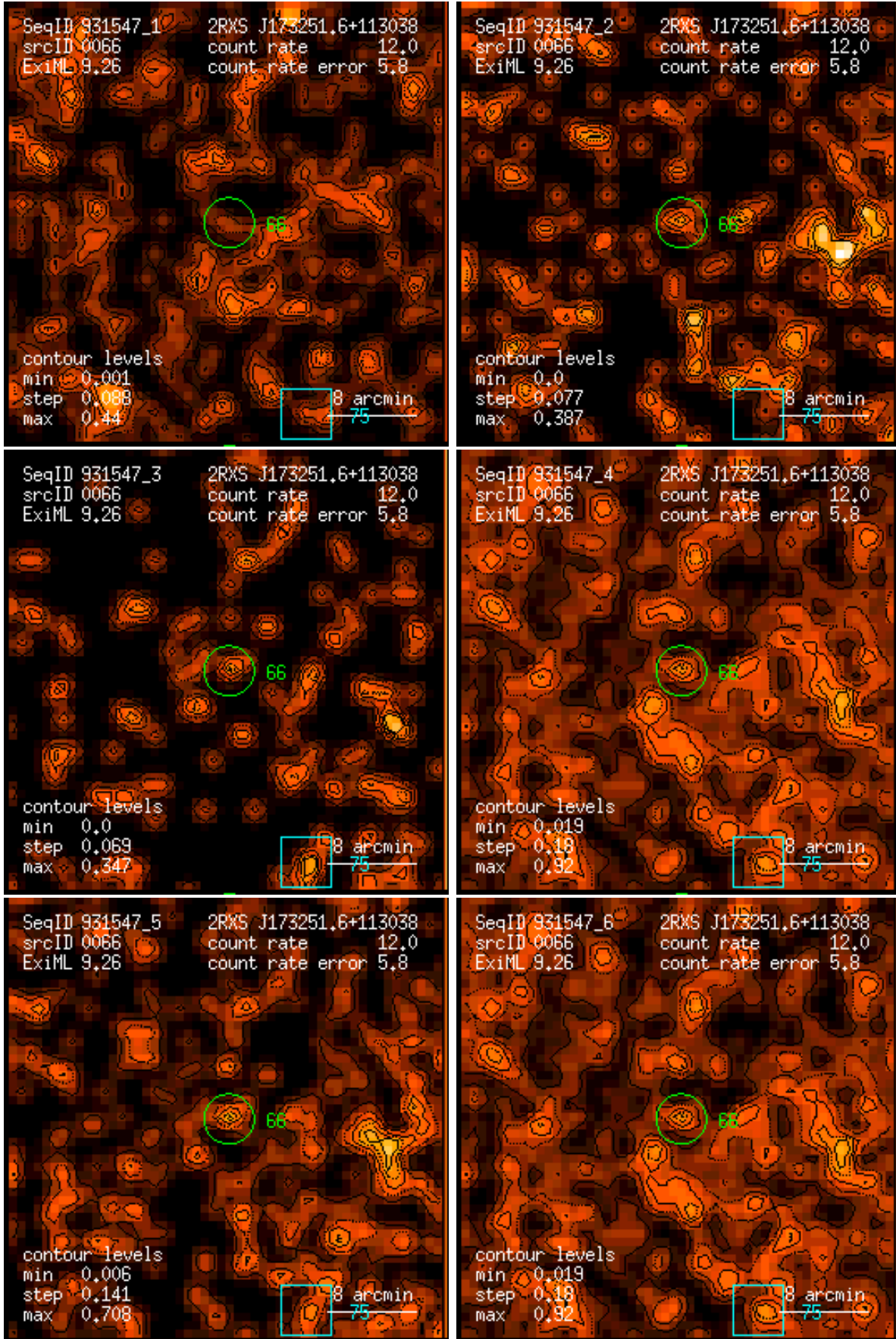
Figure 66: RASS 931547: detection 0066: band rate images, Gaussian filter: (1) PSPC channels 11 – 41, (2) 52 – 90, (3) 91 – 201, (4) 11 – 235, (5) 52 – 201, (6) 11 – 201. Broad band rates in counts/ks. Band rate contour levels in counts/ks/arcmin 2 .
