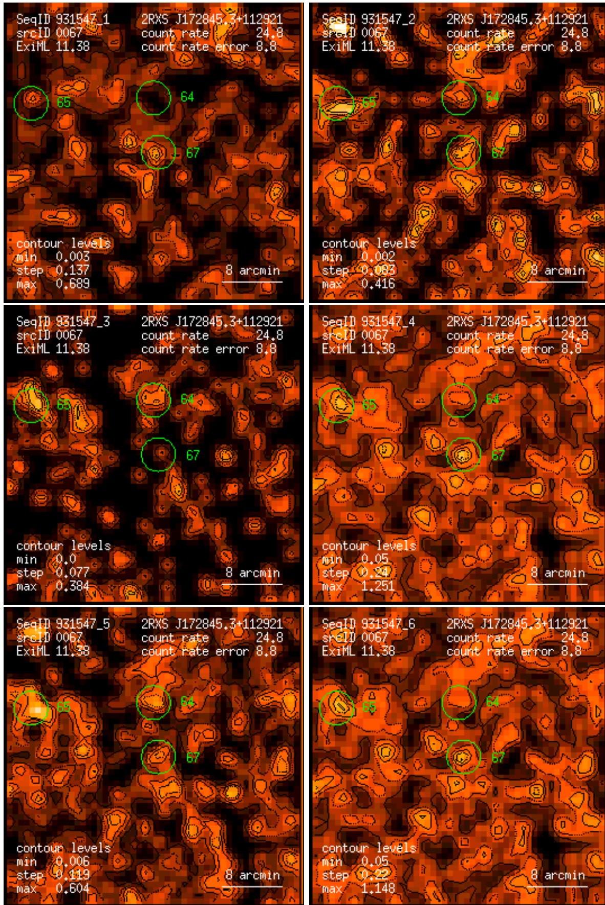
Figure 67: RASS 931547: detection 0067: band rate images, Gaussian filter: (1) PSPC channels 11 – 41, (2) 52 – 90, (3) 91 – 201, (4) 11 – 235, (5) 52 – 201, (6) 11 – 201. Broad band rates in counts/ks. Band rate contour levels in counts/ks/arcmin 2 .
