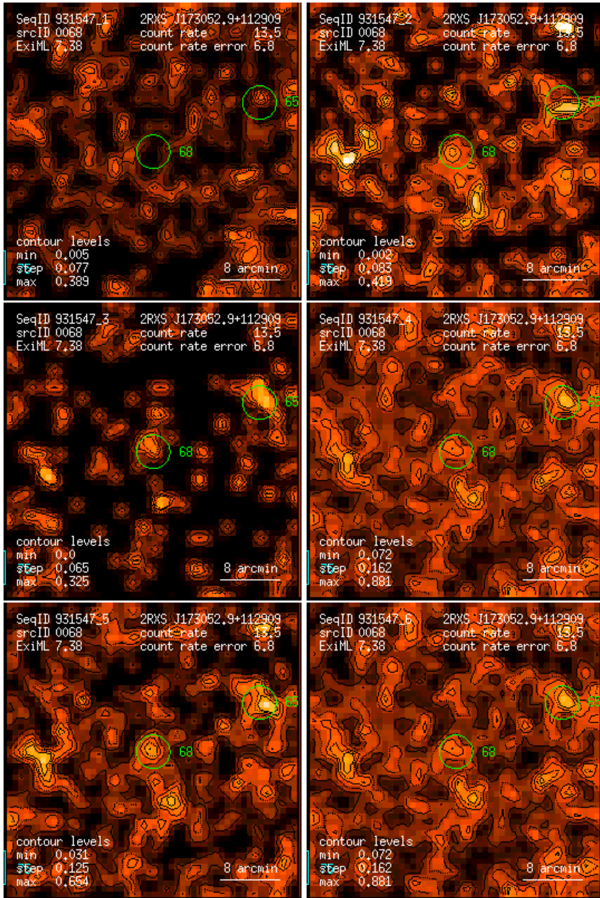
Figure 68: RASS 931547: detection 0068: band rate images, Gaussian filter: (1) PSPC channels 11 – 41, (2) 52 – 90, (3) 91 – 201, (4) 11 – 235, (5) 52 – 201, (6) 11 – 201. Broad band rates in counts/ks. Band rate contour levels in counts/ks/arcmin 2 .
