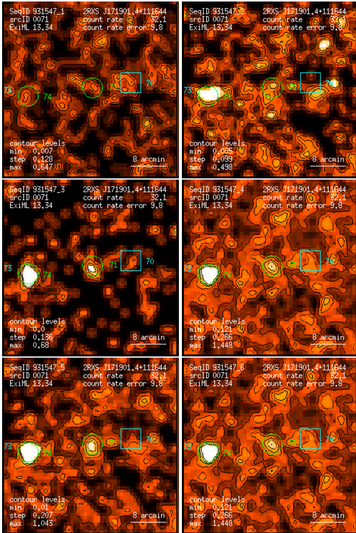
Figure 71: RASS 931547: detection 0071: band rate images, Gaussian filter: (1) PSPC channels 11 – 41, (2) 52 – 90, (3) 91 – 201, (4) 11 – 235, (5) 52 – 201, (6) 11 – 201. Broad band rates in counts/ks. Band rate contour levels in counts/ks/arcmin 2 .
