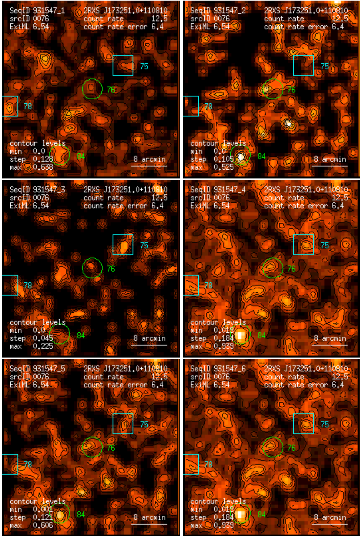
Figure 76: RASS 931547: detection 0076: band rate images, Gaussian filter: (1) PSPC channels 11 – 41, (2) 52 – 90, (3) 91 – 201, (4) 11 – 235, (5) 52 – 201, (6) 11 – 201. Broad band rates in counts/ks. Band rate contour levels in counts/ks/arcmin 2 .
