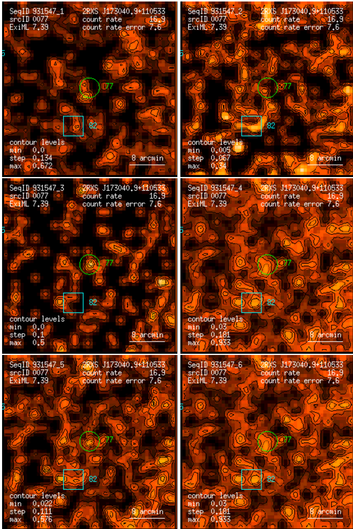
Figure 77: RASS 931547: detection 0077: band rate images, Gaussian filter: (1) PSPC channels 11 – 41, (2) 52 – 90, (3) 91 – 201, (4) 11 – 235, (5) 52 – 201, (6) 11 – 201. Broad band rates in counts/ks. Band rate contour levels in counts/ks/arcmin 2 .
