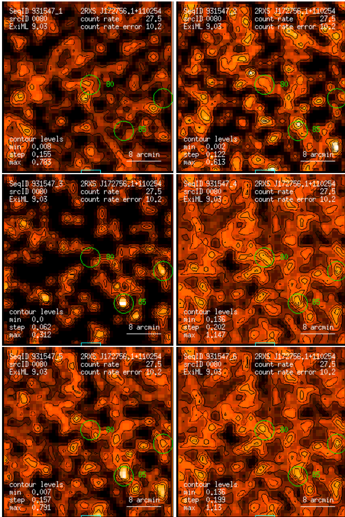
Figure 80: RASS 931547: detection 0080: band rate images, Gaussian filter: (1) PSPC channels 11 – 41, (2) 52 – 90, (3) 91 – 201, (4) 11 – 235, (5) 52 – 201, (6) 11 – 201. Broad band rates in counts/ks. Band rate contour levels in counts/ks/arcmin 2 .
