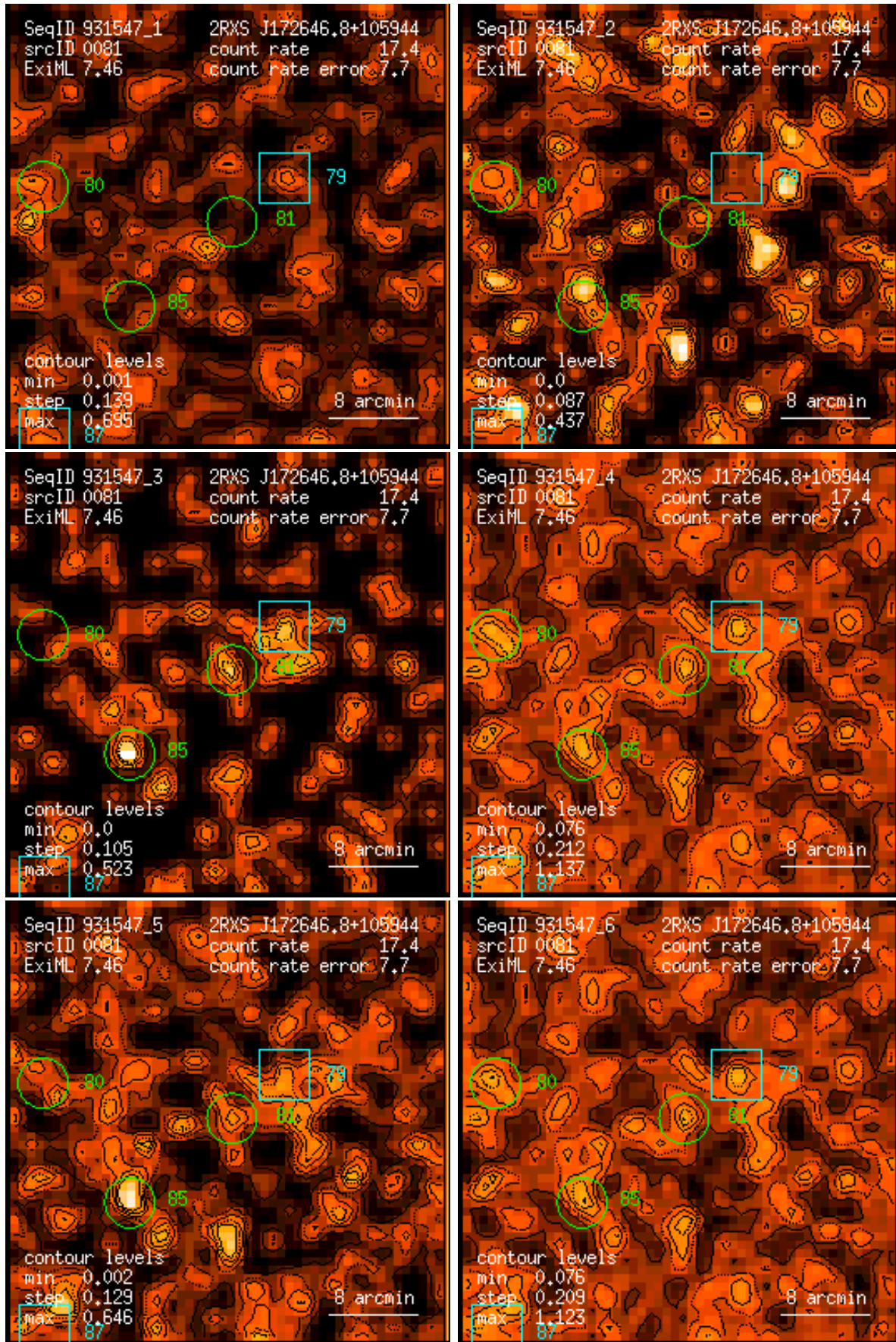
Figure 81: RASS 931547: detection 0081: band rate images, Gaussian filter: (1) PSPC channels 11 – 41, (2) 52 – 90, (3) 91 – 201, (4) 11 – 235, (5) 52 – 201, (6) 11 – 201. Broad band rates in counts/ks. Band rate contour levels in counts/ks/arcmin 2 .
