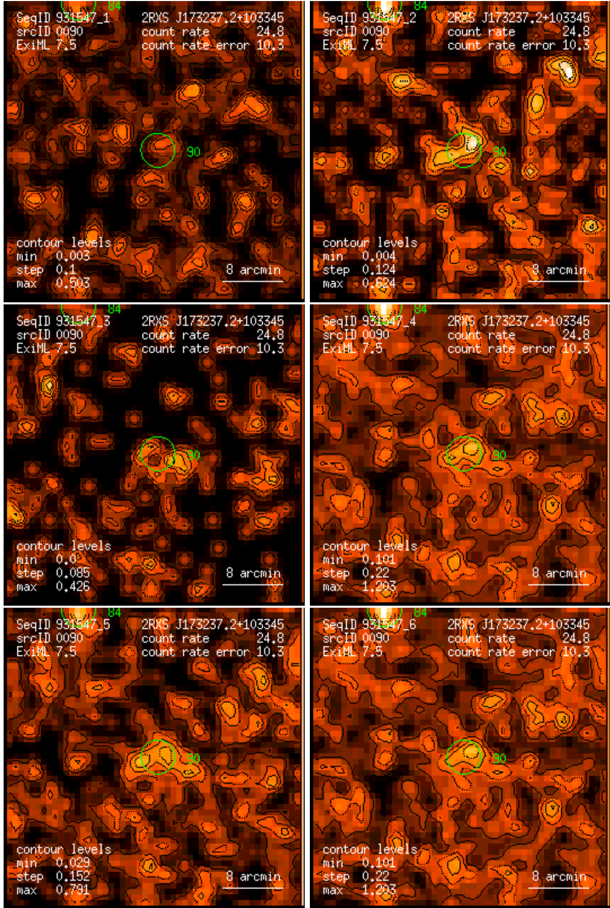
Figure 90: RASS 931547: detection 0090: band rate images, Gaussian filter: (1) PSPC channels 11 – 41, (2) 52 – 90, (3) 91 – 201, (4) 11 – 235, (5) 52 – 201, (6) 11 – 201. Broad band rates in counts/ks. Band rate contour levels in counts/ks/arcmin 2 .
