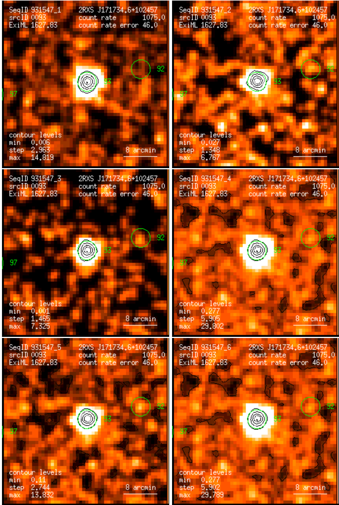
Figure 93: RASS 931547: detection 0093: band rate images, Gaussian filter: (1) PSPC channels 11 – 41, (2) 52 – 90, (3) 91 – 201, (4) 11 – 235, (5) 52 – 201, (6) 11 – 201. Broad band rates in counts/ks. Band rate contour levels in counts/ks/arcmin 2 .
