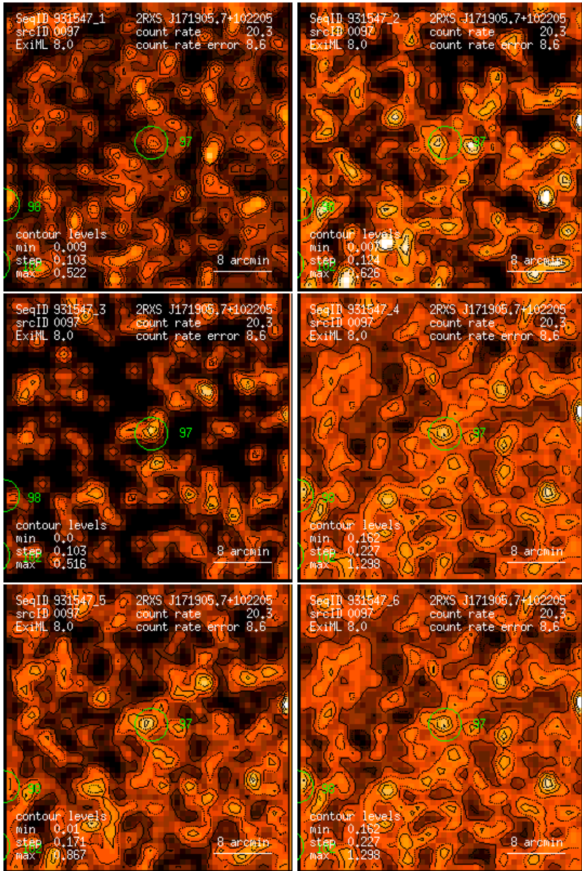
Figure 97: RASS 931547: detection 0097: band rate images, Gaussian filter: (1) PSPC channels 11 – 41, (2) 52 – 90, (3) 91 – 201, (4) 11 – 235, (5) 52 – 201, (6) 11 – 201. Broad band rates in counts/ks. Band rate contour levels in counts/ks/arcmin 2 .
