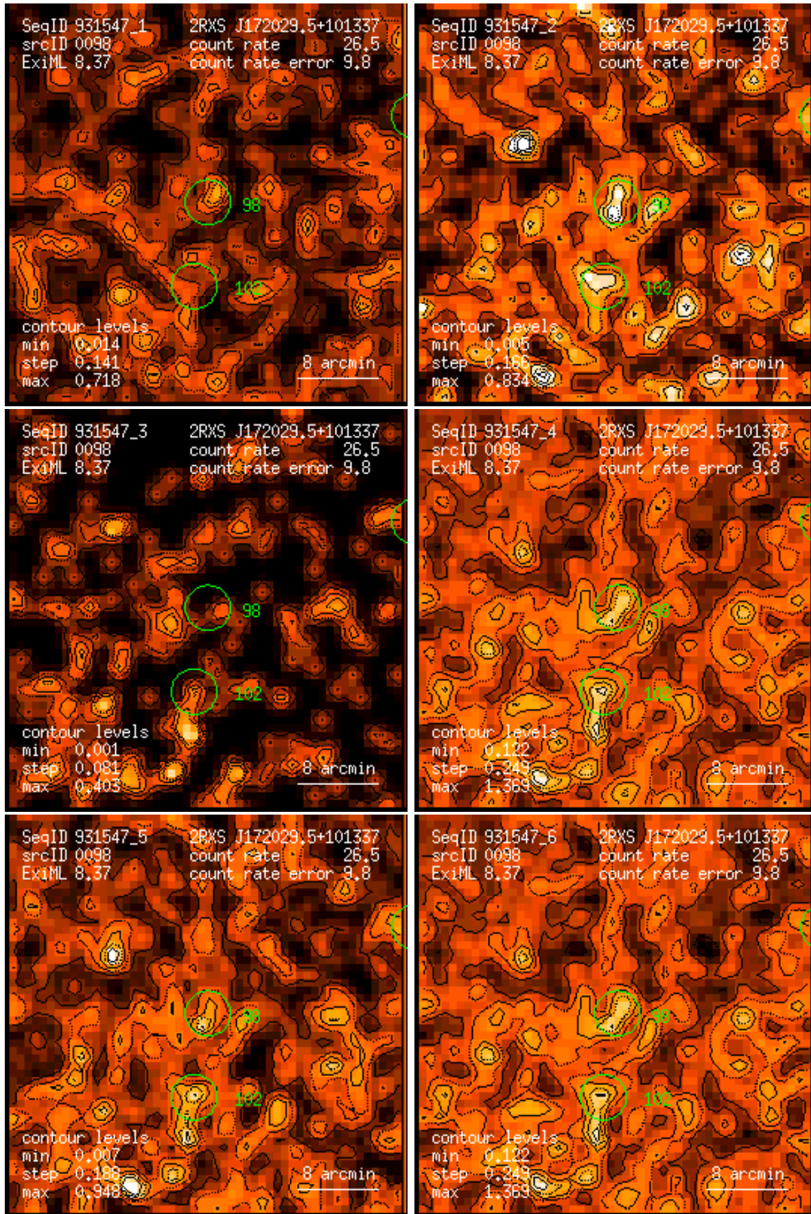
Figure 98: RASS 931547: detection 0098: band rate images, Gaussian filter: (1) PSPC channels 11 – 41, (2) 52 – 90, (3) 91 – 201, (4) 11 – 235, (5) 52 – 201, (6) 11 – 201. Broad band rates in counts/ks. Band rate contour levels in counts/ks/arcmin 2 .
