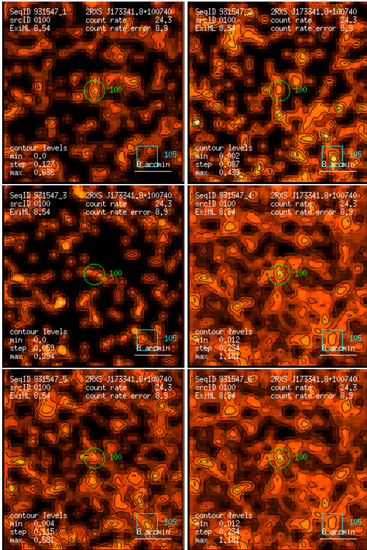
Figure 100: RASS 931547: detection 0100: band rate images, Gaussian filter: (1) PSPC channels 11 – 41, (2) 52 – 90, (3) 91 – 201, (4) 11 – 235, (5) 52 – 201, (6) 11 – 201. Broad band rates in counts/ks. Band rate contour levels in counts/ks/arcmin 2 .
