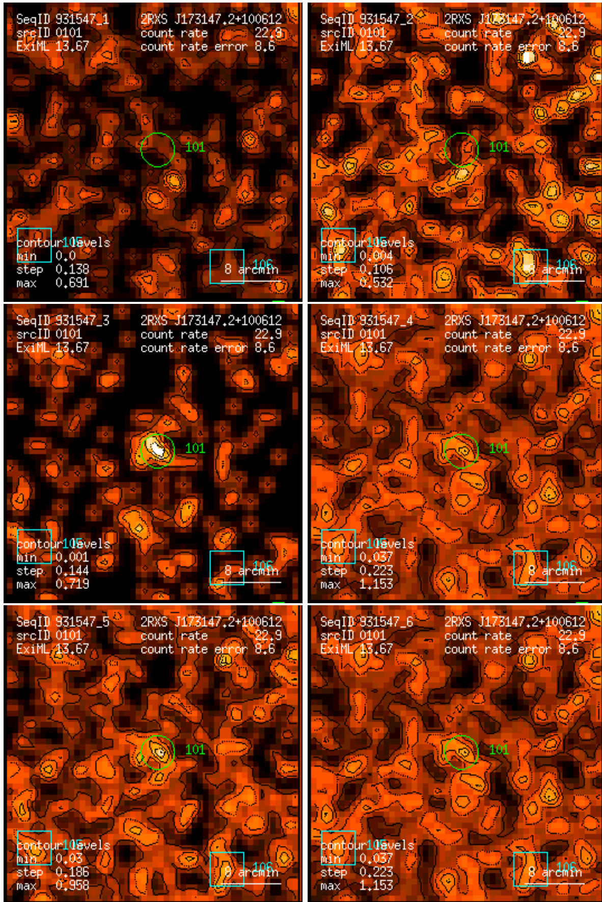
Figure 101: RASS 931547: detection 0101: band rate images, Gaussian filter: (1) PSPC channels 11 – 41, (2) 52 – 90, (3) 91 – 201, (4) 11 – 235, (5) 52 – 201, (6) 11 – 201. Broad band rates in counts/ks. Band rate contour levels in counts/ks/arcmin 2 .
