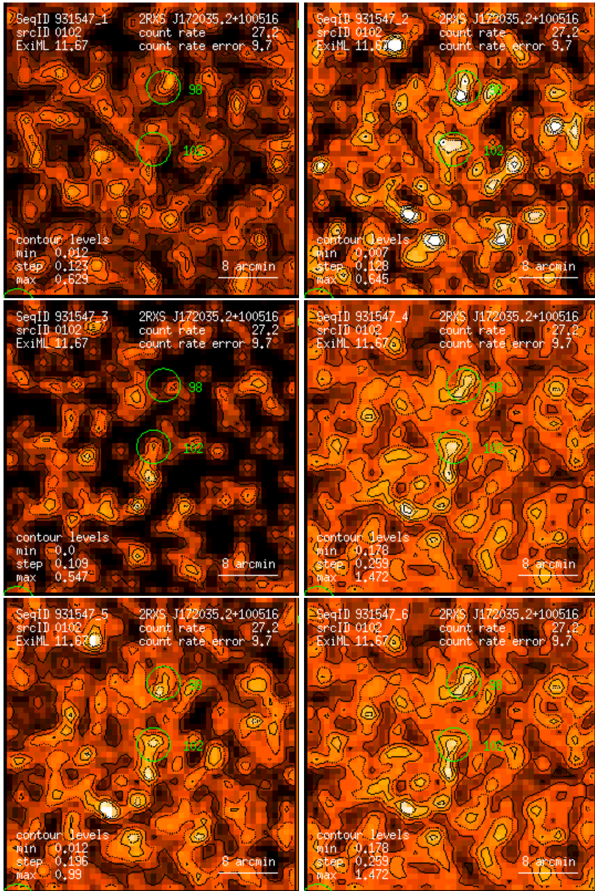
Figure 102: RASS 931547: detection 0102: band rate images, Gaussian filter: (1) PSPC channels 11 – 41, (2) 52 – 90, (3) 91 – 201, (4) 11 – 235, (5) 52 – 201, (6) 11 – 201. Broad band rates in counts/ks. Band rate contour levels in counts/ks/arcmin 2 .
