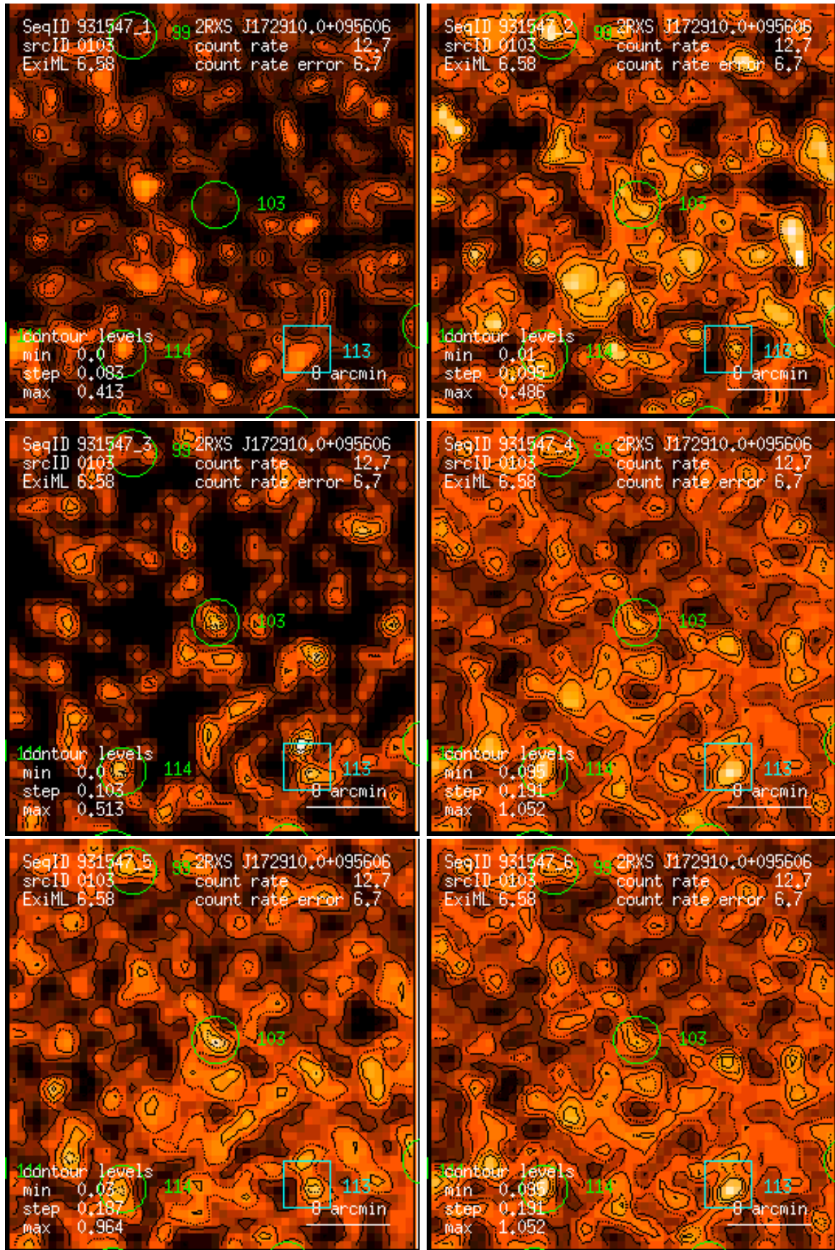
Figure 103: RASS 931547: detection 0103: band rate images, Gaussian filter: (1) PSPC channels 11 – 41, (2) 52 – 90, (3) 91 – 201, (4) 11 – 235, (5) 52 – 201, (6) 11 – 201. Broad band rates in counts/ks. Band rate contour levels in counts/ks/arcmin 2 .
