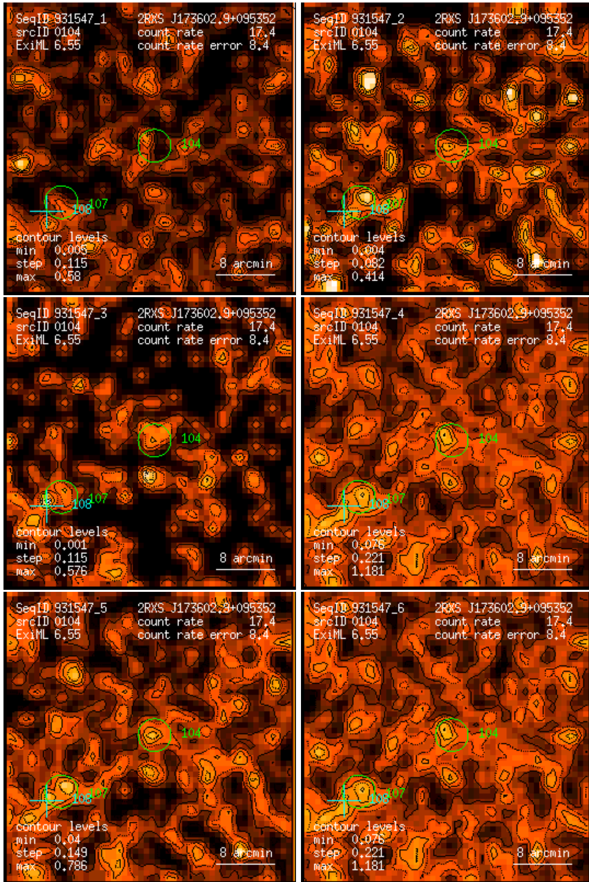
Figure 104: RASS 931547: detection 0104: band rate images, Gaussian filter: (1) PSPC channels 11 – 41, (2) 52 – 90, (3) 91 – 201, (4) 11 – 235, (5) 52 – 201, (6) 11 – 201. Broad band rates in counts/ks. Band rate contour levels in counts/ks/arcmin 2 .
