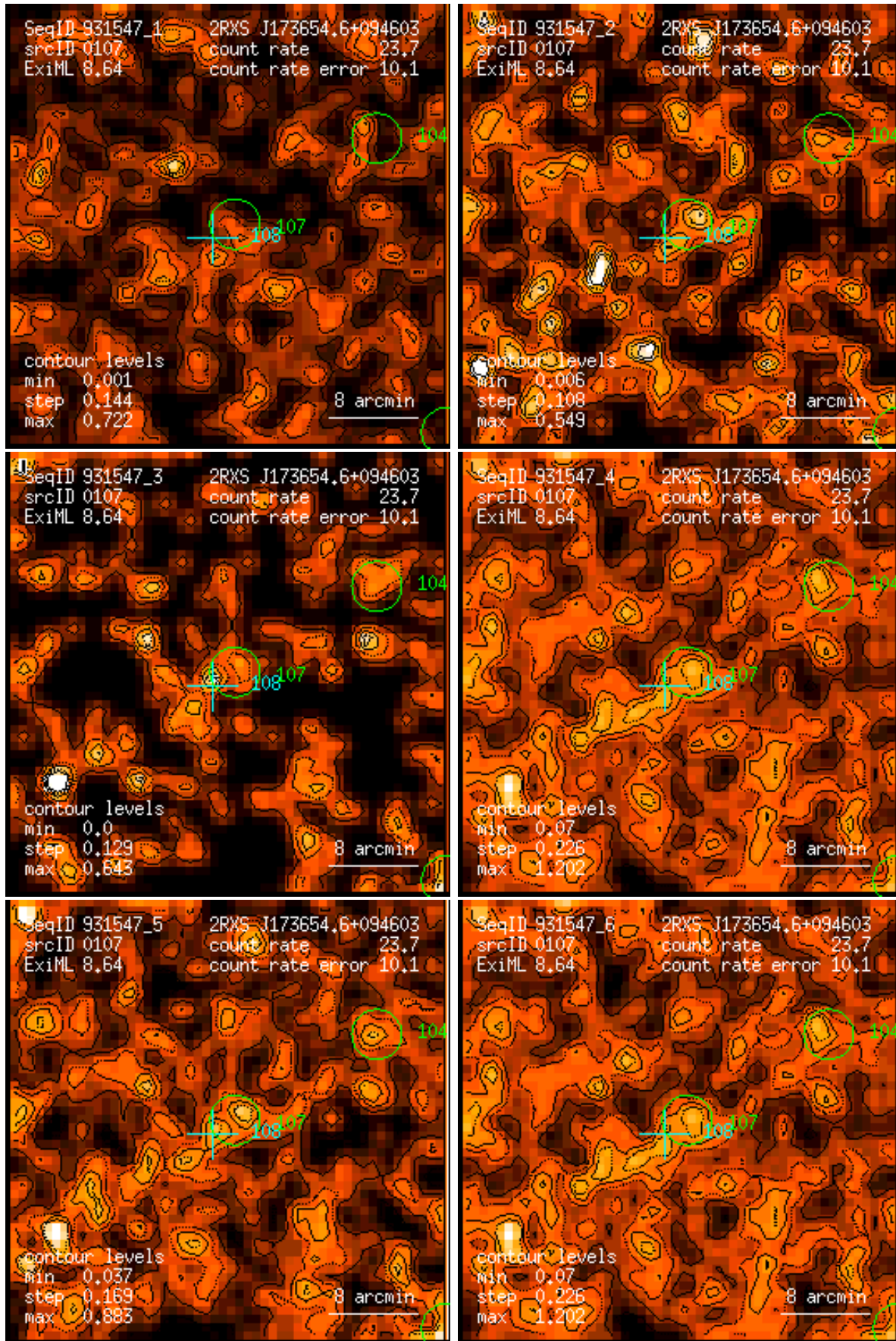
Figure 107: RASS 931547: detection 0107: band rate images, Gaussian filter: (1) PSPC channels 11 – 41, (2) 52 – 90, (3) 91 – 201, (4) 11 – 235, (5) 52 – 201, (6) 11 – 201. Broad band rates in counts/ks. Band rate contour levels in counts/ks/arcmin 2 .
