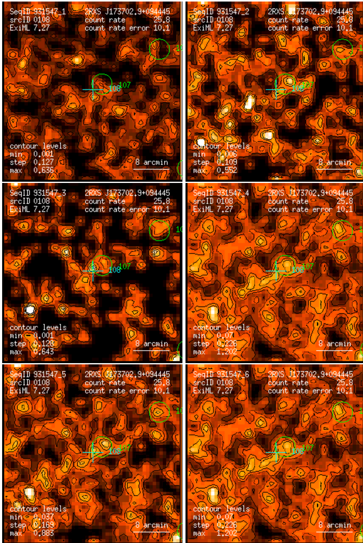
Figure 108: RASS 931547: detection 0108: band rate images, Gaussian filter: (1) PSPC channels 11 – 41, (2) 52 – 90, (3) 91 – 201, (4) 11 – 235, (5) 52 – 201, (6) 11 – 201. Broad band rates in counts/ks. Band rate contour levels in counts/ks/arcmin 2 .
